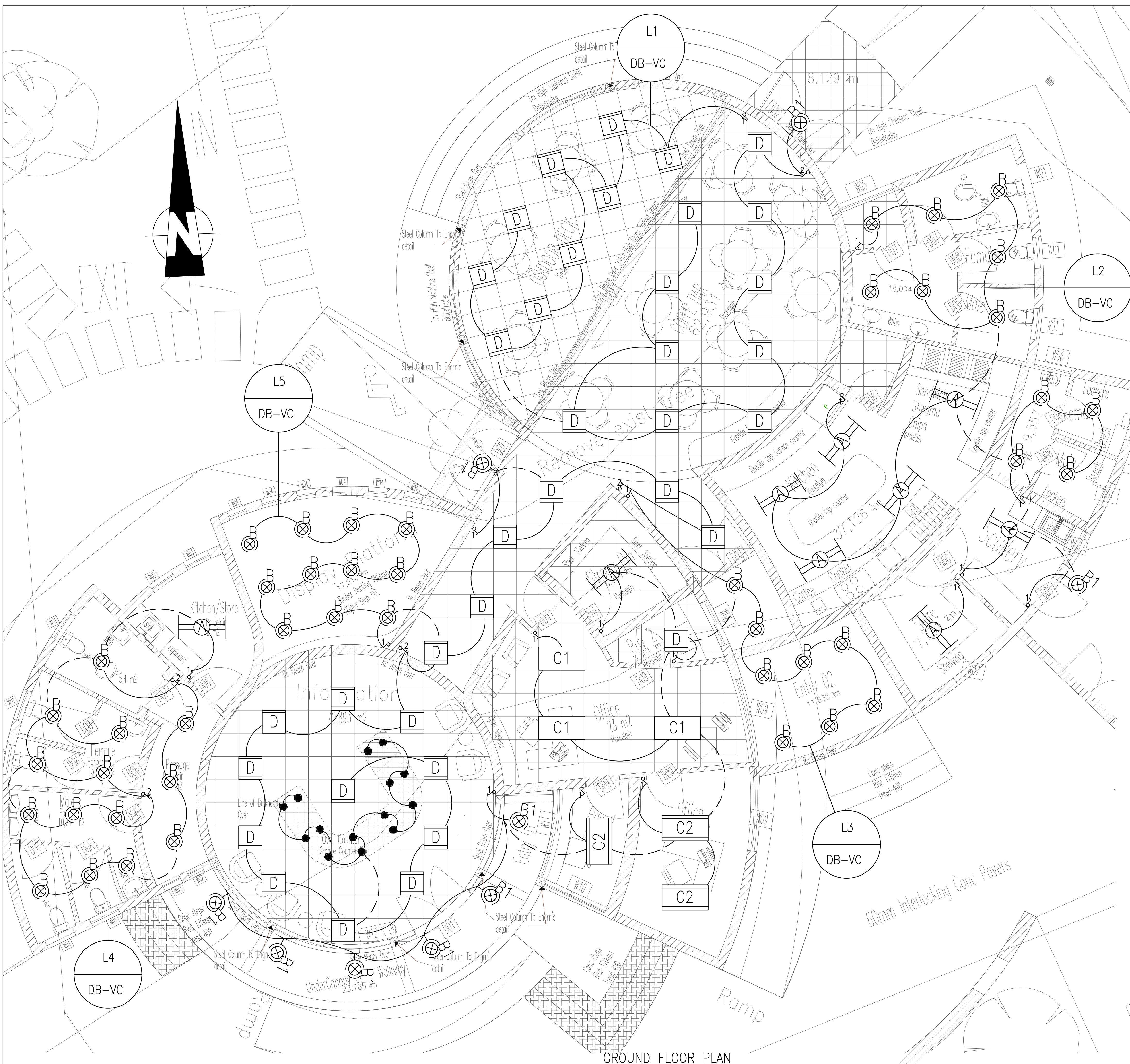
GROUND FLOOR PLAN SCALE 1:50
