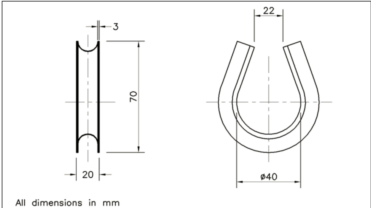
Figure 2 – Thimble
