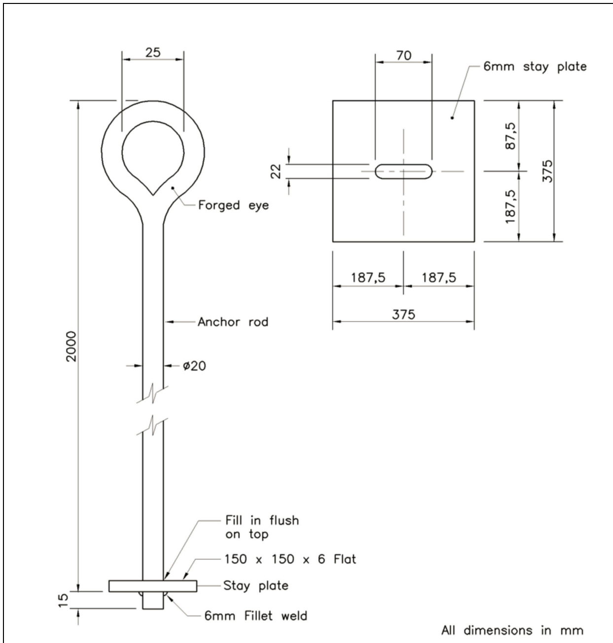
Figure 1 - Stay-anchor
