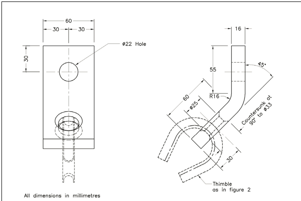
Figure 5 – Stay strap
