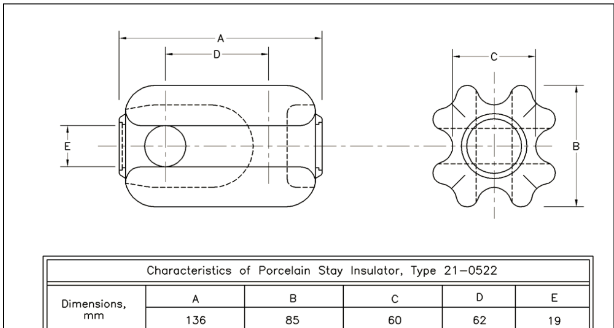
Figure 3 – Typical porcelain stay insulator
