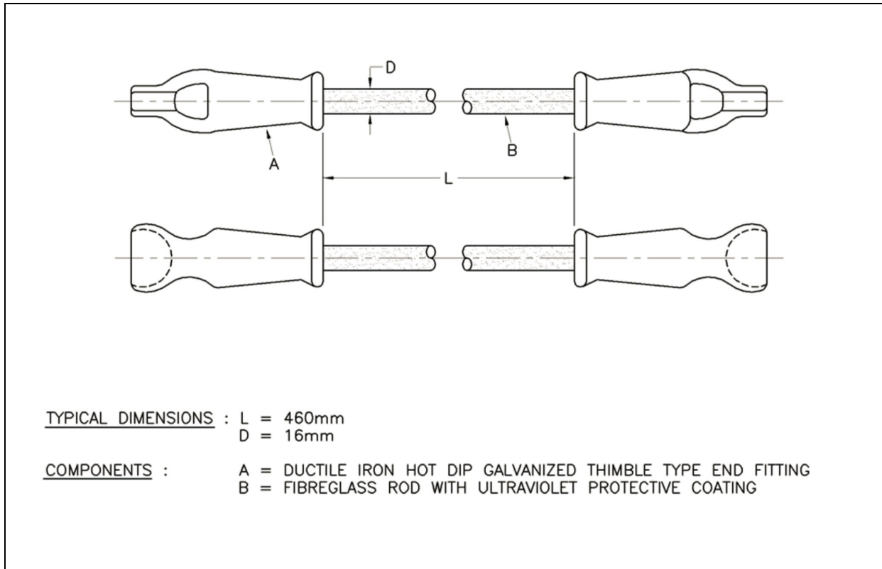
Figure 4 – Typical guy strain stay insulator
