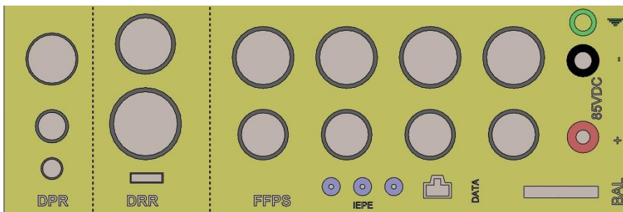
Figure 1-8 The interface on the Main Cabinet panel sidewall
