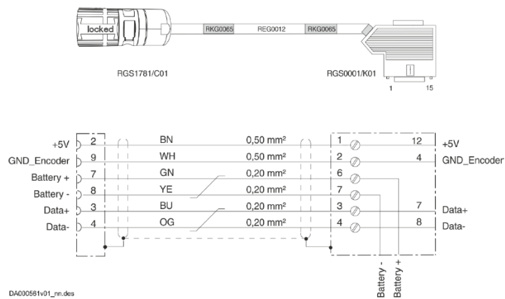
Figure 1-10 Encoder Cable diagram for the TVM DRR
