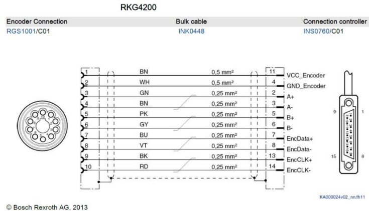
Figure 1-6 DRR Motor Encoder Cable
