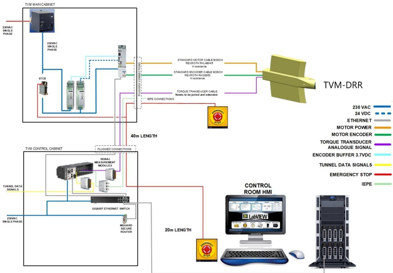
Figure 1-9 Overview of the Control wiring for the TVM-500 Rig
