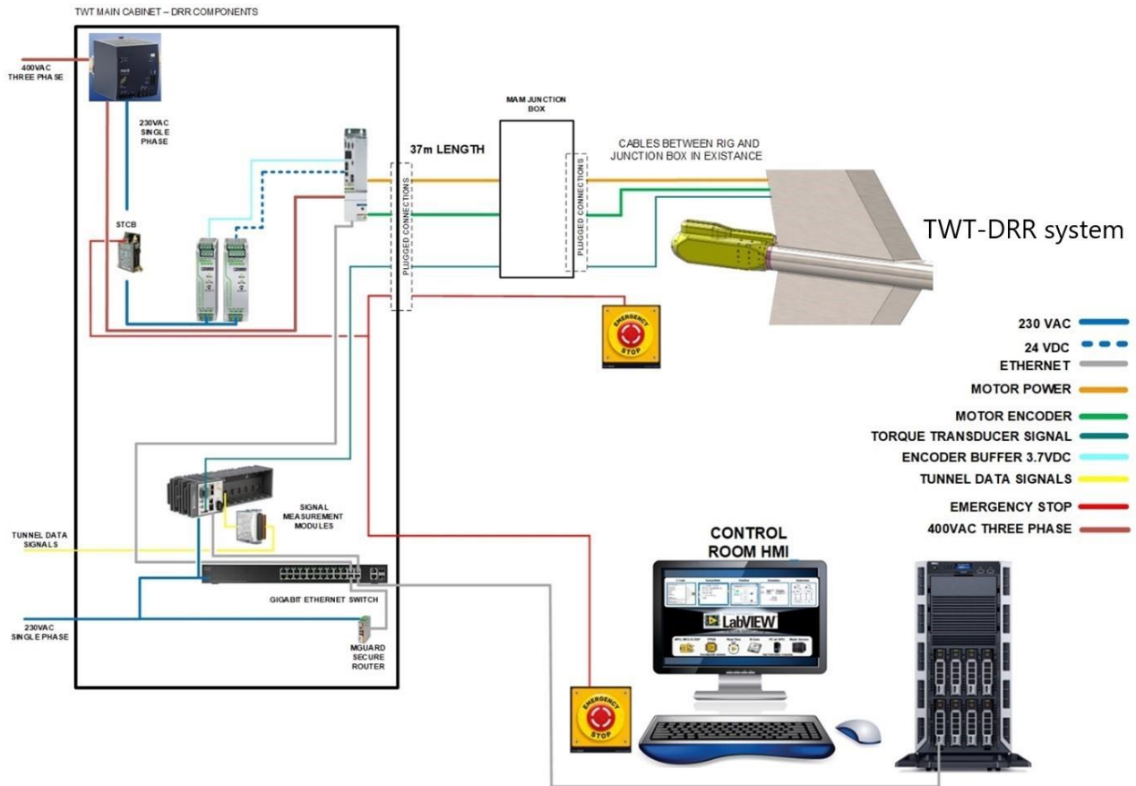
Figure 1-2 Dynamic Roll Rig wiring schematic showing the core elements.
