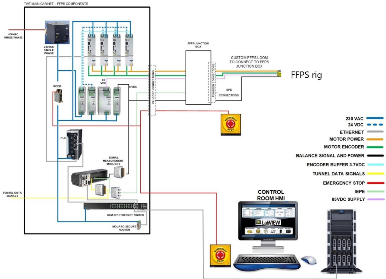
Figure 1-3 FFPS wiring schematic showing the core elements.
