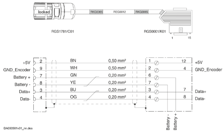
Figure 1-5 Encoder Cable Specifications
