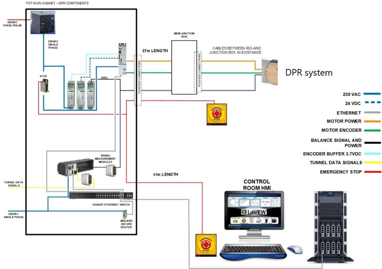
Figure 1-1 Dynamic Pitch Rig wiring schematic showing the core elements.
