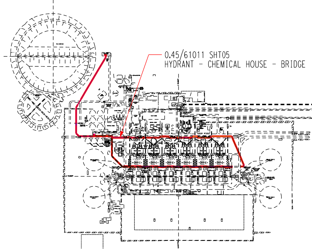
PLOT PLAN
