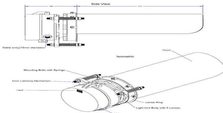
Figure 1 - 152mm Housing
