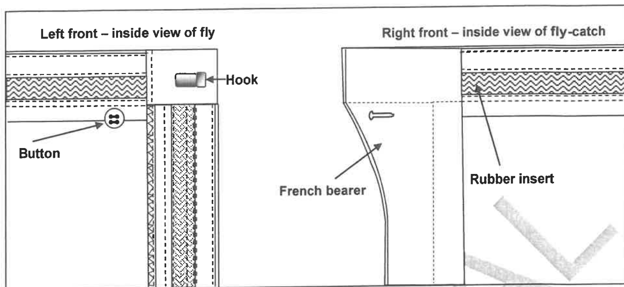
Figure 4 – Inside view of fly and fly-catch
