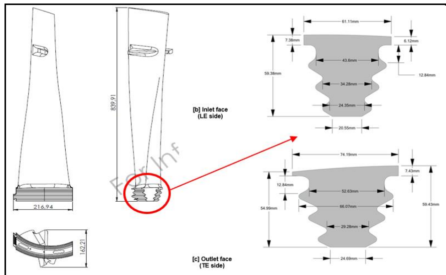
Figure 1 – Kusile/Medupi LP last stage blade sketch showing details of the root
