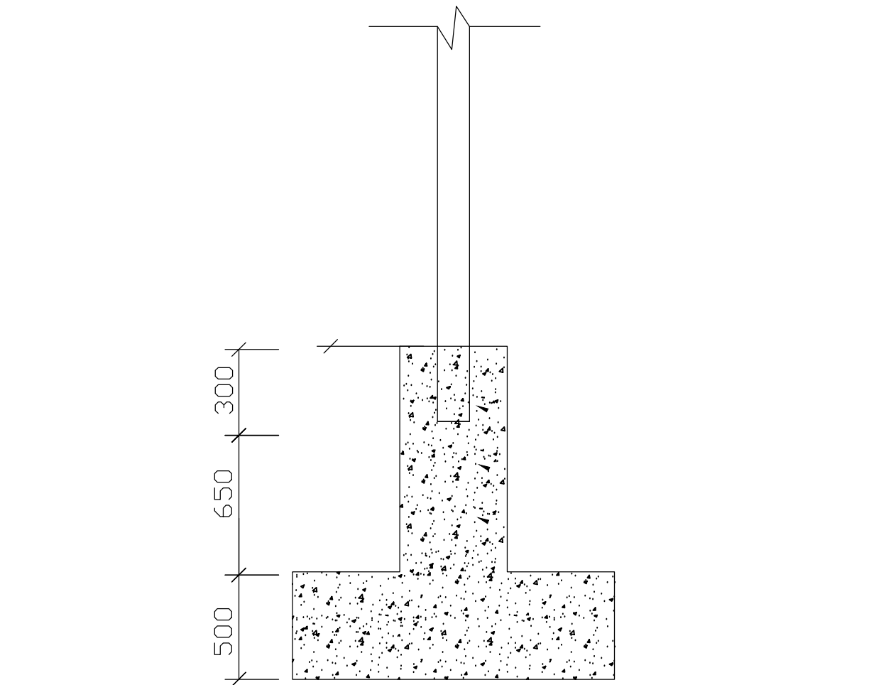
FOUNDATION SECTION
