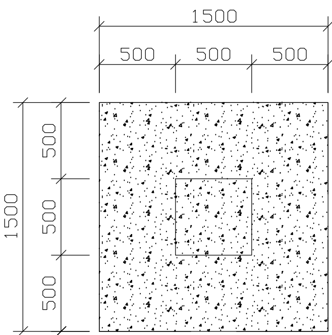
FOUNDATION LAYOUT
