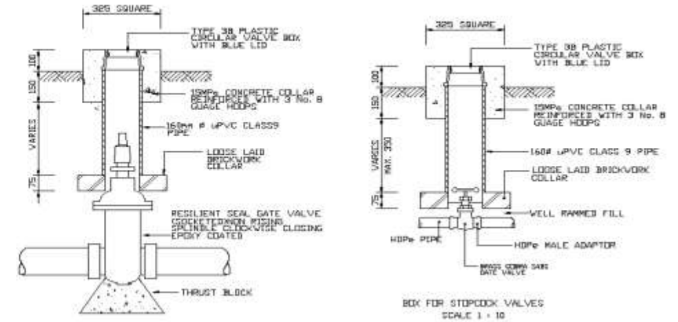
VALVE BOX FOR INLINE WATER WORKS VALVES UP TO 75mm DIA
