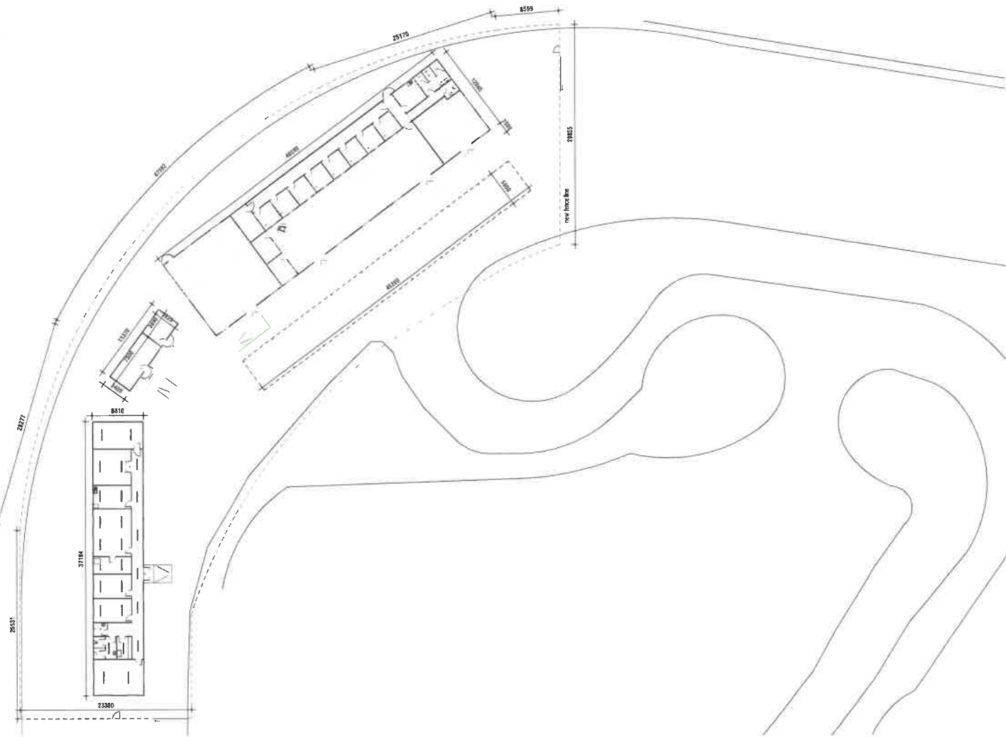
2 | GROUND FLOOR PLAN 1 : 250
