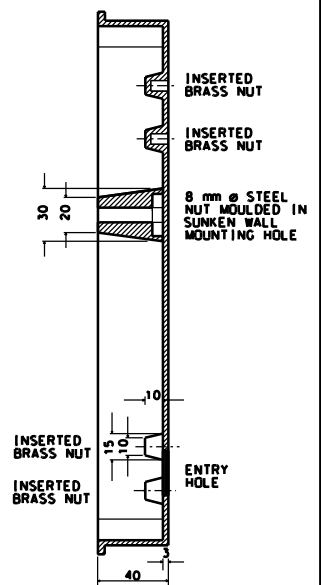
SIDE VIEW ( CUT AWAY )
