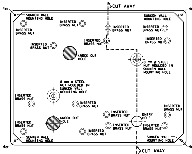
REAR VIEW
