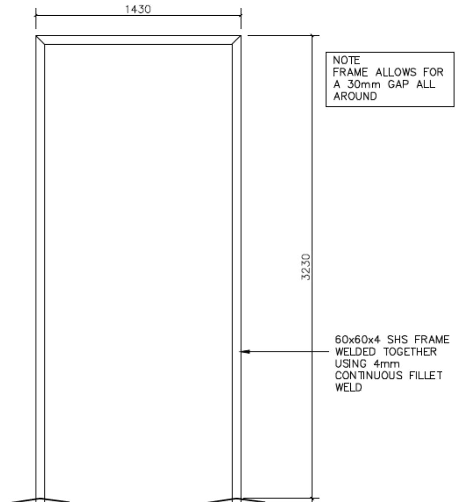
Typical Frame (NTS)
