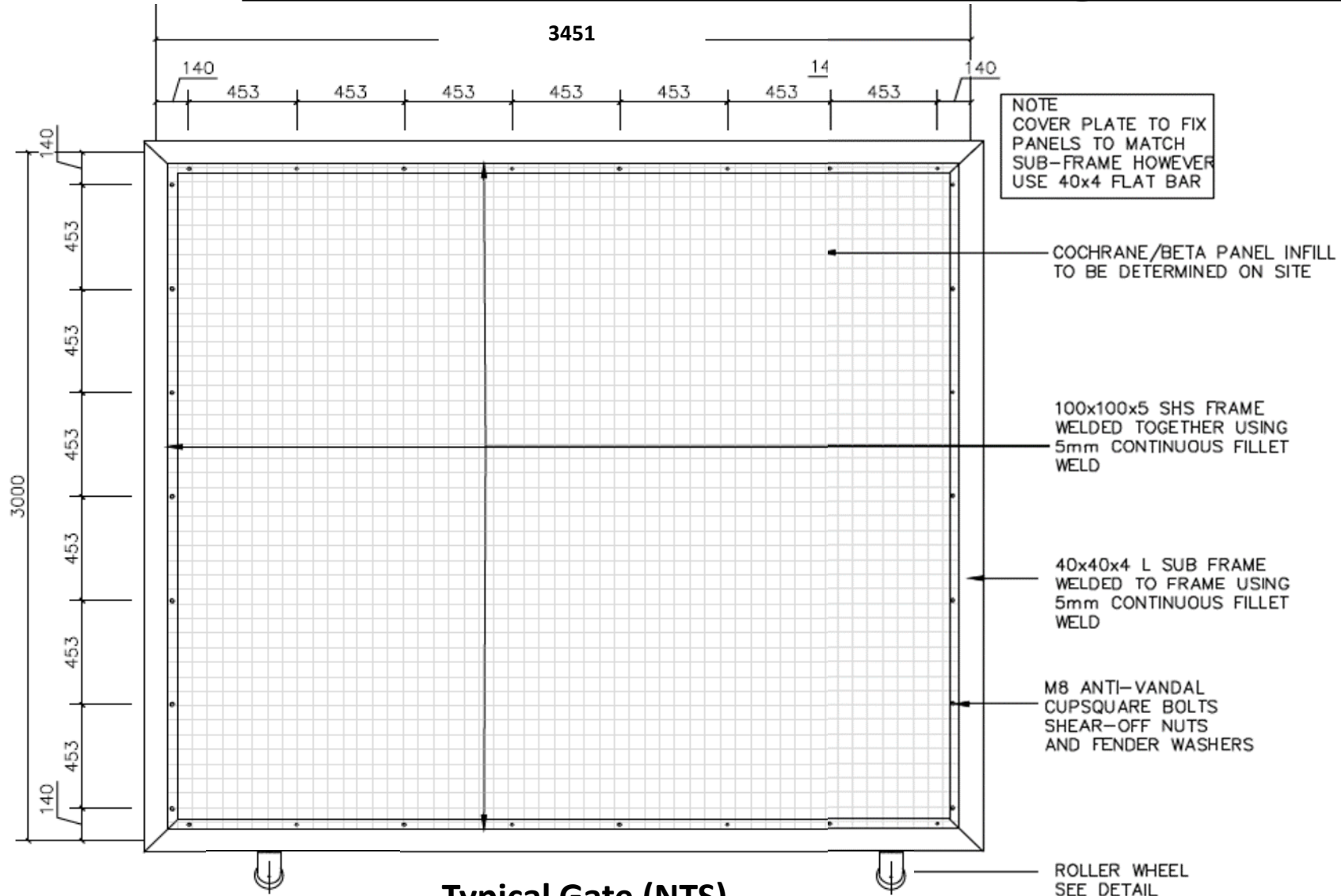
Typical Gate (NTS)
