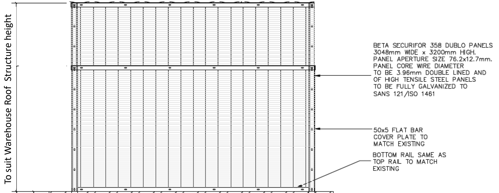
Typical Fence Beta Fence (NTS)
