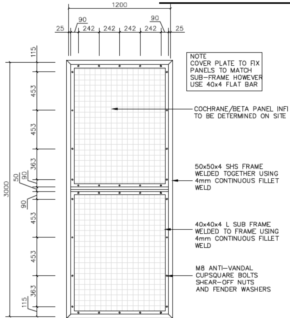
Typical Gate (NTS)
