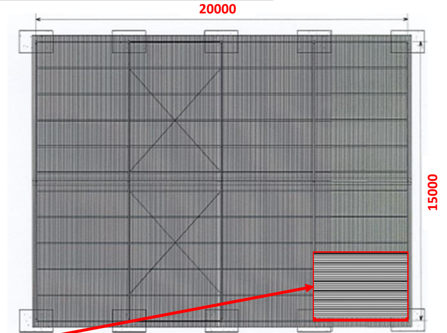
Roof Plan (NTS)
