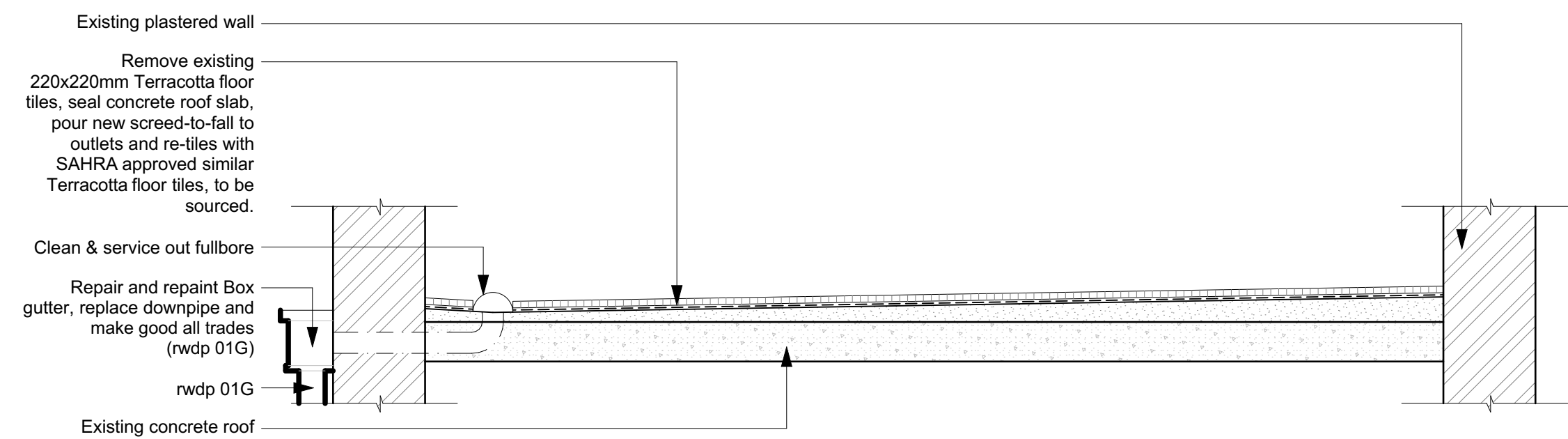
Detail 100-01 - TYPICAL BALCONY DETAIL Scale 1:10
