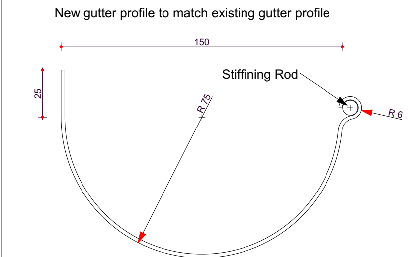
Detail 100-03 - GUTTER DETAIL Scale 1:2
