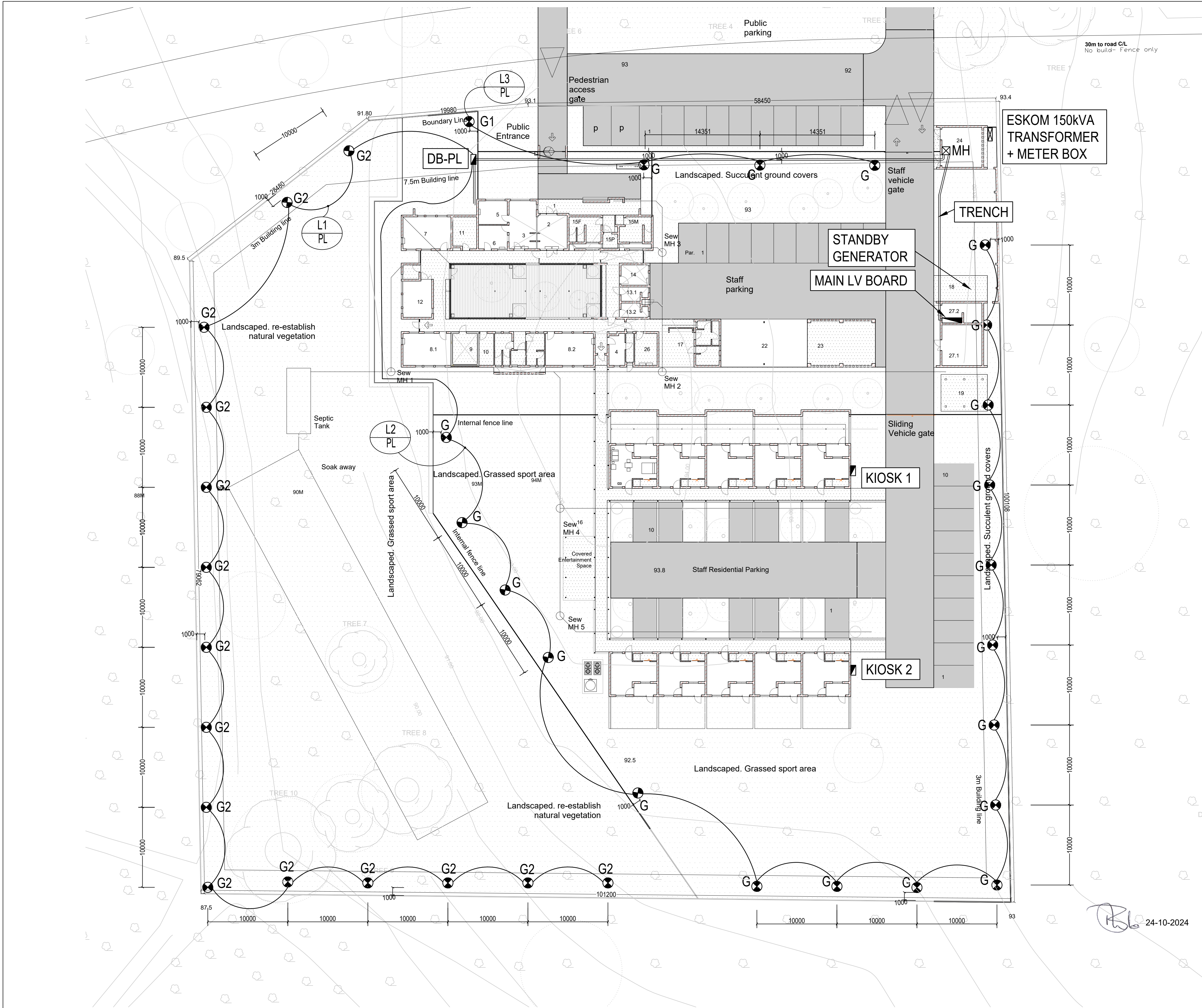
SITE DEVELOPMENT PLAN CABLE RETICULATION AND STREET LIGHTING LAYOUT SCALE 1:250
