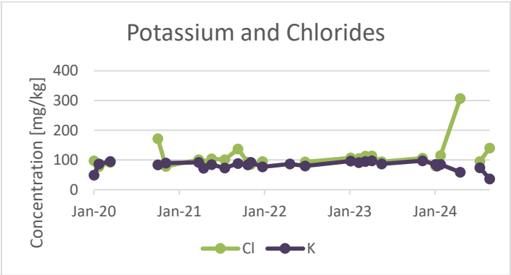
Figure 37: Kriel Ash water Potassium and Chloride concentration
