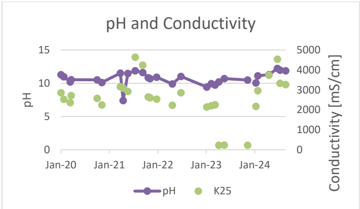
Figure 33: Kriel Ash Water pH and Conductivity
