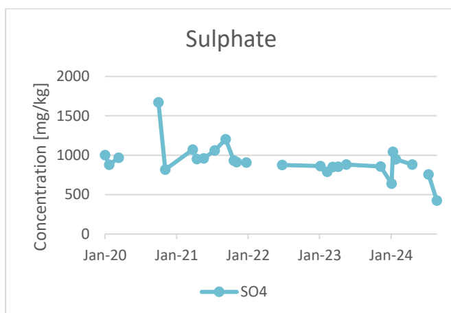
Figure 39: Kriel Ash water sulphate concentration
