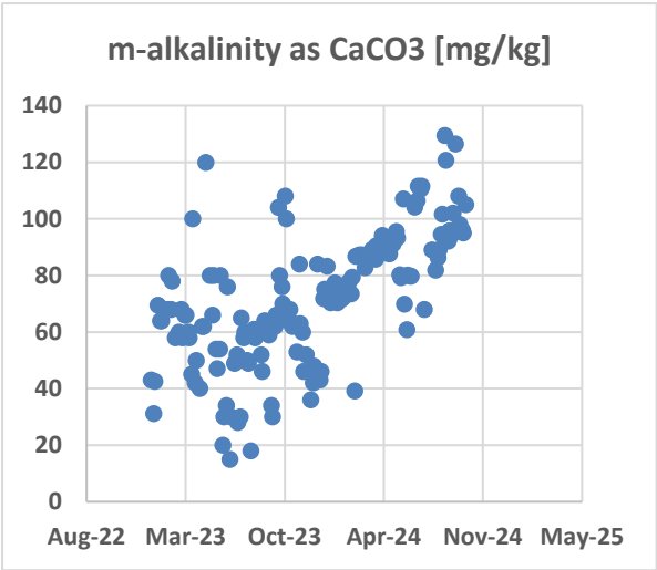
Figure 4: Raw water m-alkalinity
