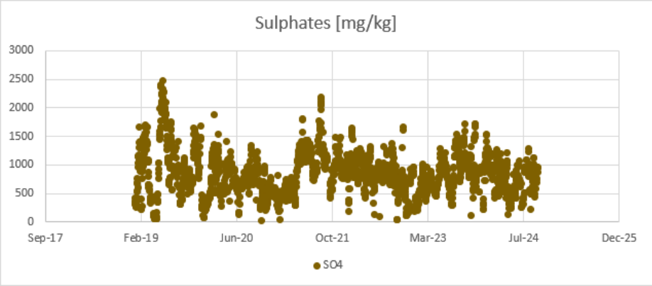
Figure 59: Kriel Cooling water South pH and sulphate
