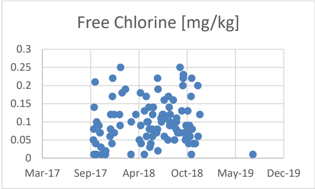
Figure 47: Tutuka SRO brine Free chlorine
