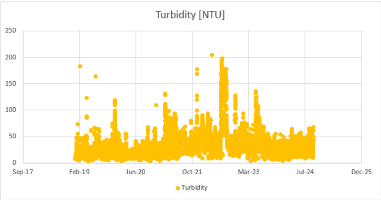
Figure 63: Kriel Cooling water North turbidity
