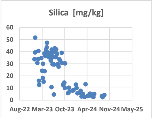
Figure 11: Raw water silica
