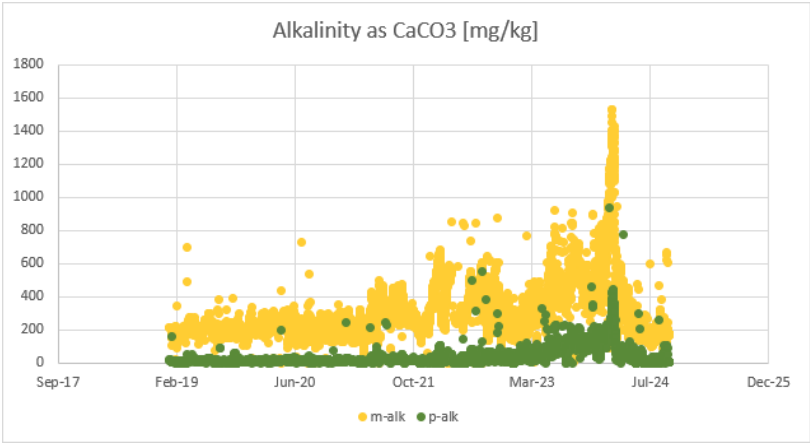
Figure 85: Tutuka Cooling water West alkalinity
