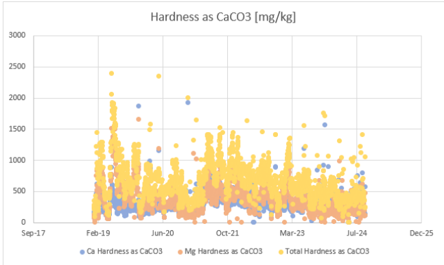
Figure 65: Kriel Cooling water North hardness
