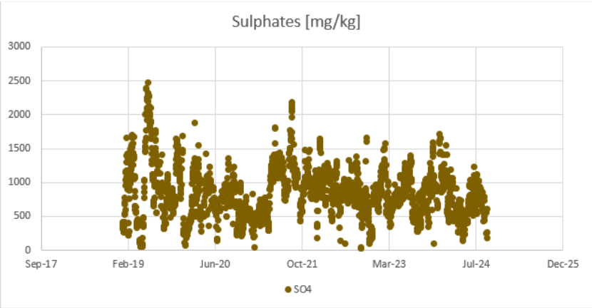
Figure 69: Kriel Cooling water North Sulphates
