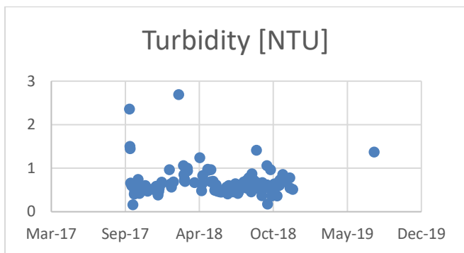
Figure 42: Tutuka SRO brine turbidity
