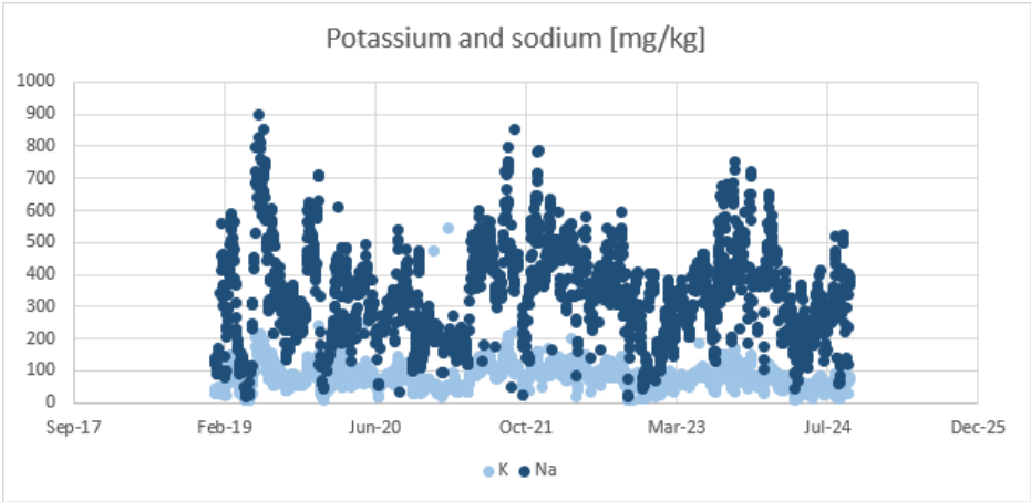
Figure 57: Kriel Cooling water South Potassium and sodium
