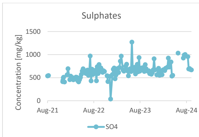
Figure 31: Duvha Ash Water Sulphates
