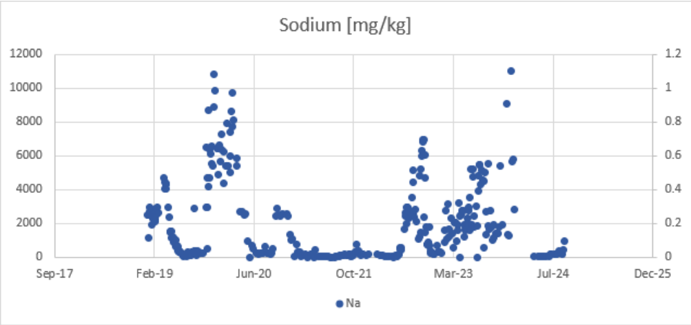
Figure 76: Tutuka Cooling water East Sodium
