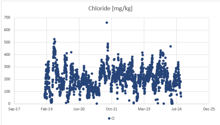
Figure 67: Kriel Cooling water North Chlorides
