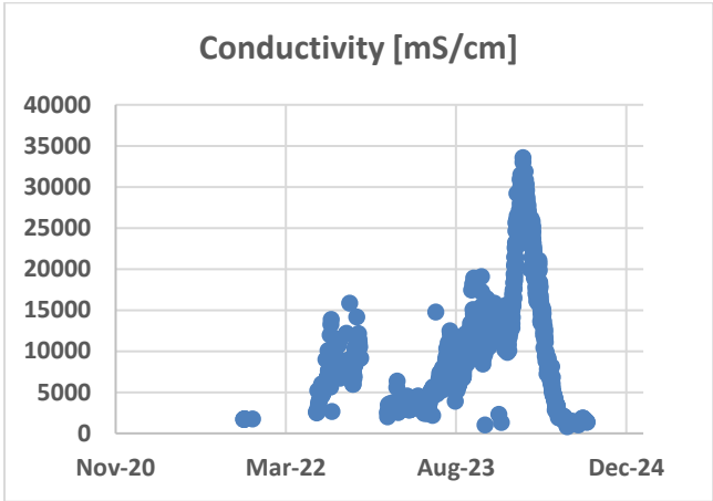
Figure 16: Dirty water dam recovery conductivity at Tutuka Power Station
