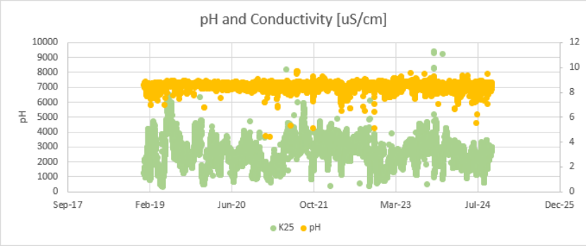
Figure 53: Kriel Cooling water South pH and conductivity
