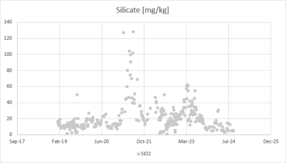
Figure 91: Tutuka Cooling water West silicates
