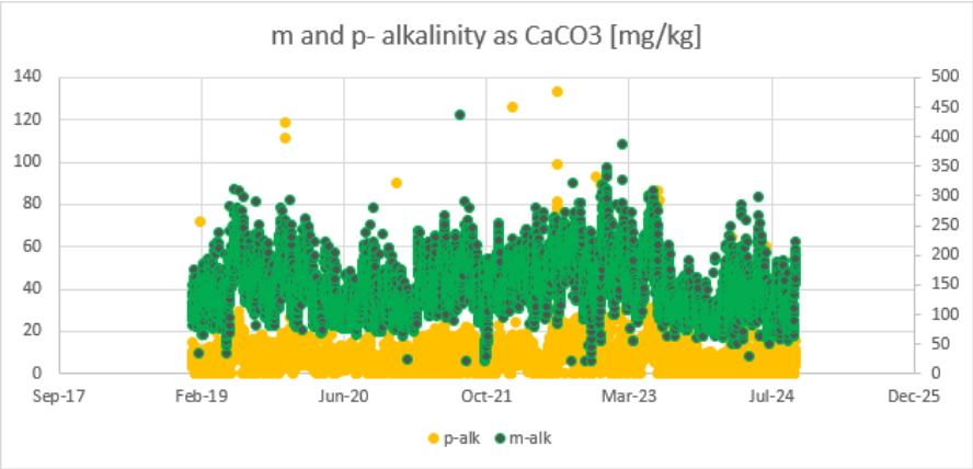
Figure 55: Kriel Cooling water South p-alkalinity and m-alkalinity
