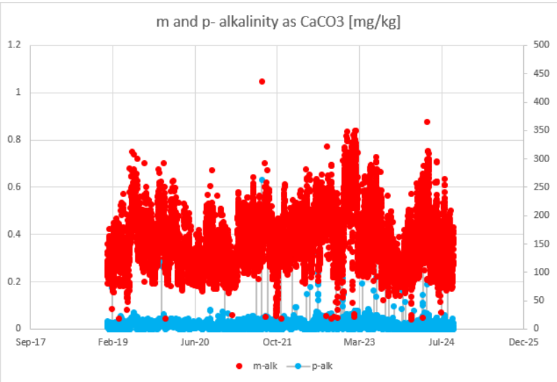
Figure 64: Kriel Cooling water North m-alkalinity and p-alkalinity
