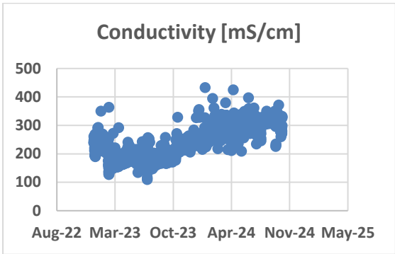
Figure 1: Raw water conductivity at Tutuka Power Station
