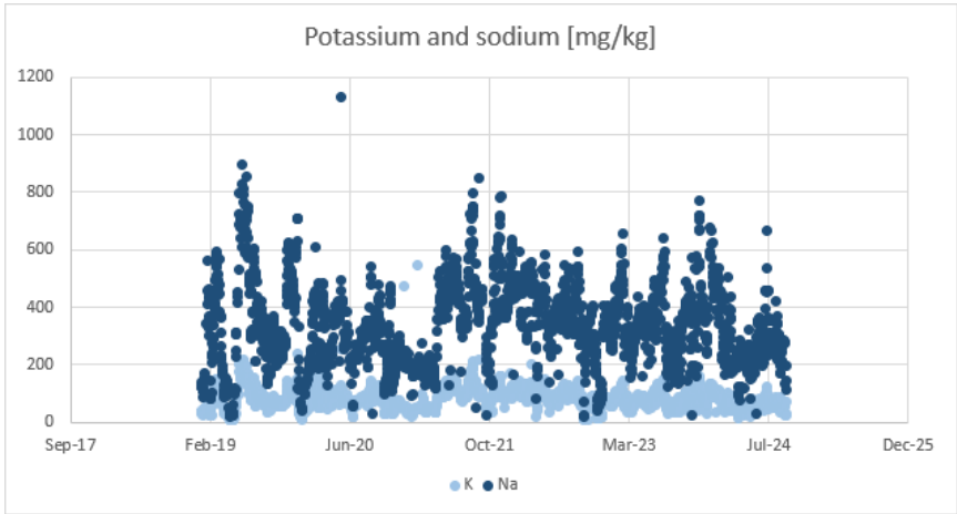
Figure 66: Kriel Cooling water North Potassium and Sodium
