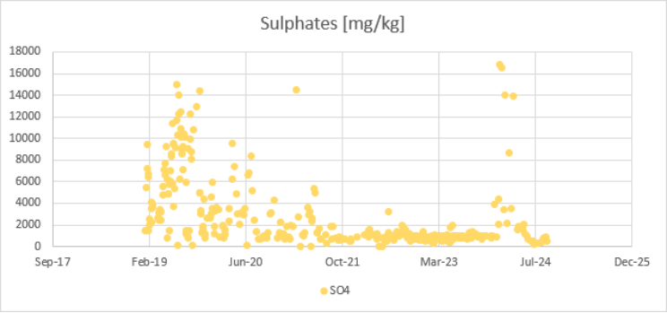
Figure 90: Tutuka Cooling water West sulfates
