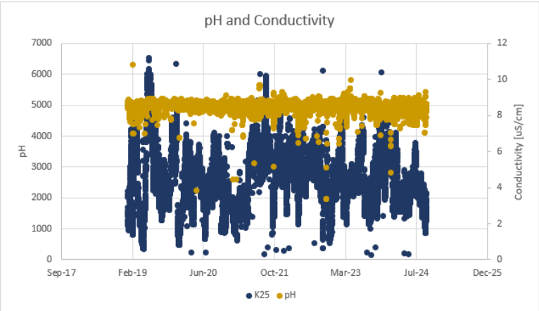
Figure 62: Kriel Cooling water North pH and conductivity
