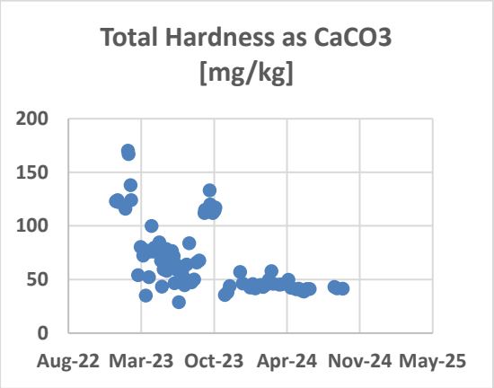
Figure 8: Raw water total hardness
