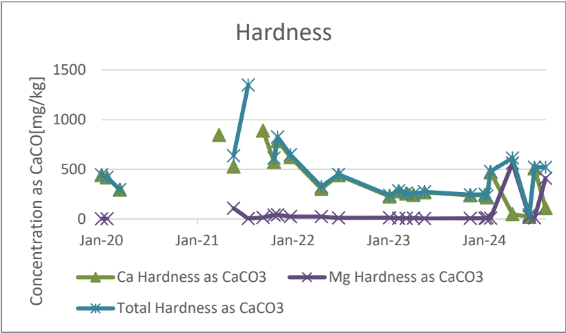
Figure 35: Kriel Ash water Hardness
