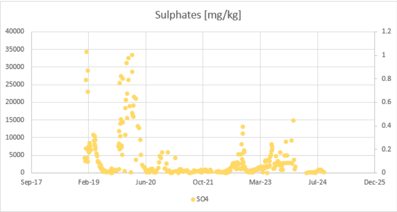
Figure 79: Tutuka Cooling water East Sulphates
