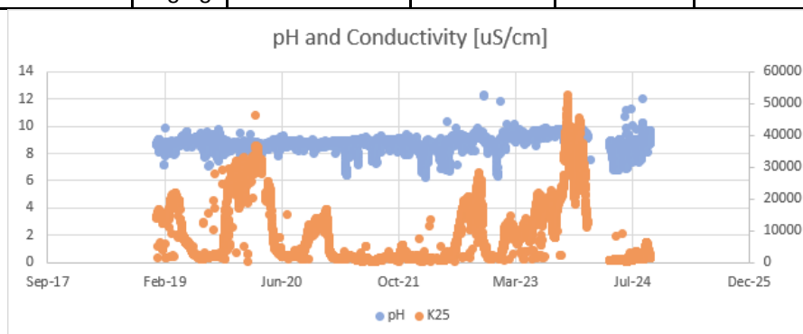
Figure 71: Tutuka Cooling water East pH and Conductivity
