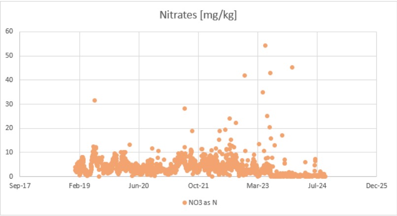
Figure 68: Kriel Cooling water North Nitrates
