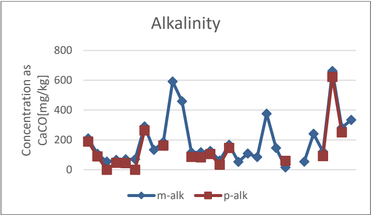
Figure 36: Kriel Ash water Alkalinity
