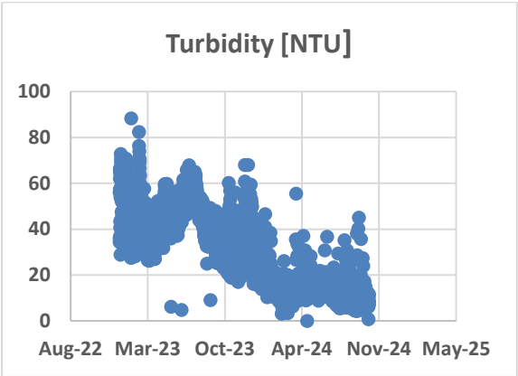
Figure 3: Raw water turbidity at Tutuka Power Station
