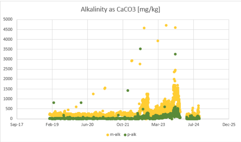
Figure 74: Tutuka Cooling water East Alkalinity
