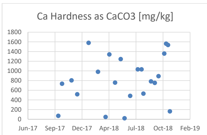
Figure 44: Tutuka SRO Calcium hardness
