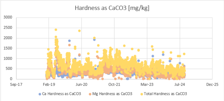
Figure 56: Kriel Cooling water South Hardness
