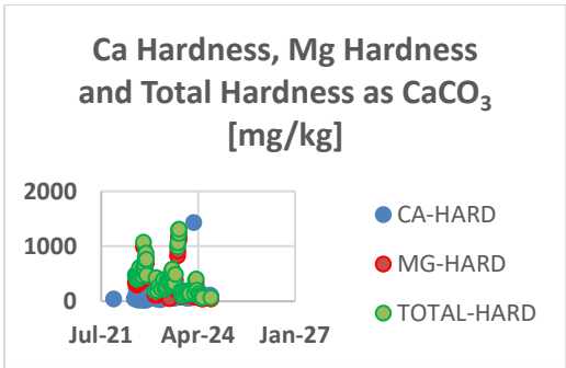
Figure 20: Dirty water dam recovery Calcium, magnesium and total hardness at Tutuka Power Station
