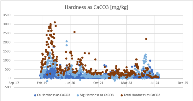
Figure 84: Tutuka Cooling water West Hardness
