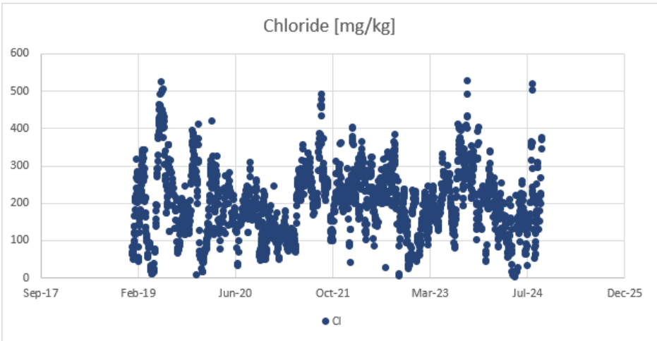
Figure 58: Kriel Cooling water South Chloride
