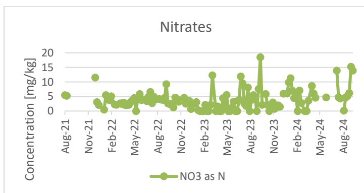
Figure 32: Duvha Ash Water Nitrates
