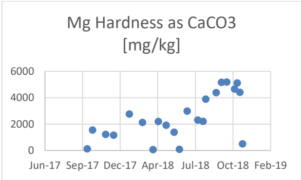
Figure 45: Tutuka SRO brine magnesium hardness
