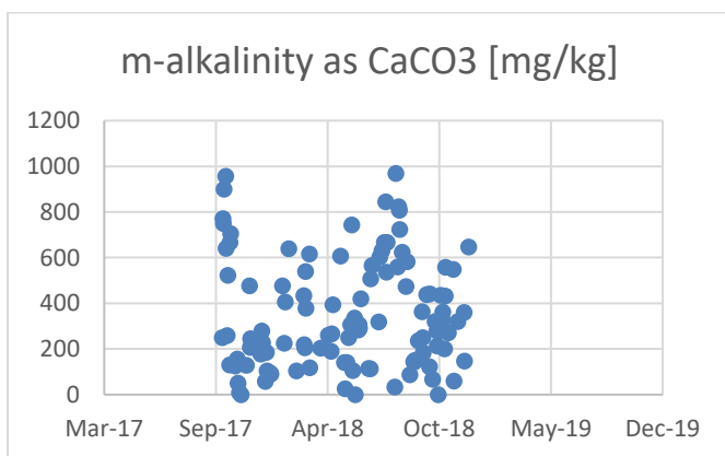
Figure 43: Tutuka SRO brine m-alkalinity
