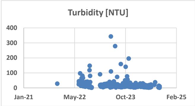
Figure 18: Dirty water dam recovery turbidity at Tutuka Power Station
