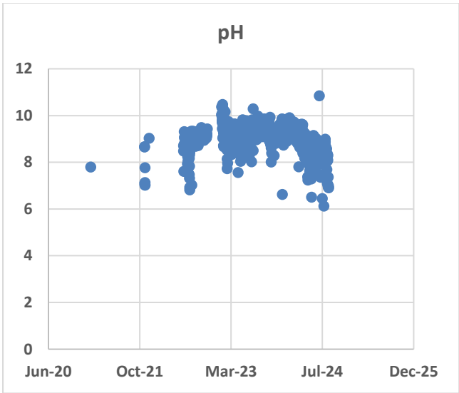
Figure 17: Dirty water dam recovery pH at Tutuka Power Station
