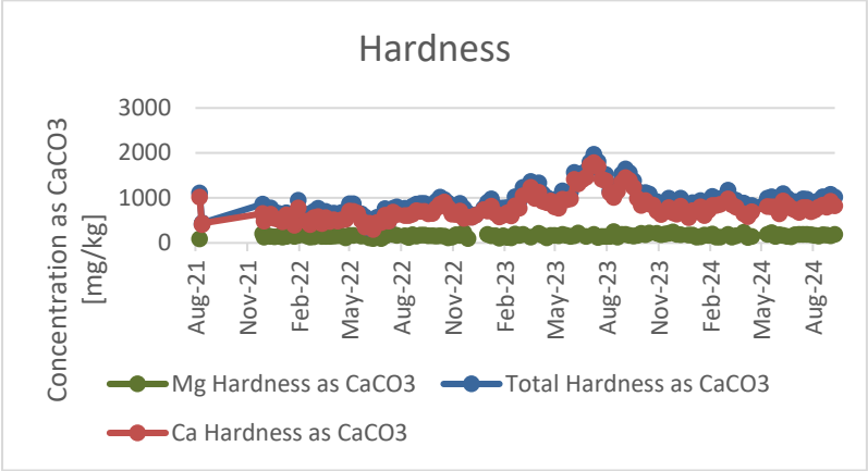
Figure 28: Duvha Ash Water Hardness
