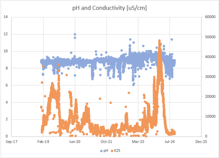
Figure 82: Tutuka Cooling water West pH and conductivity
