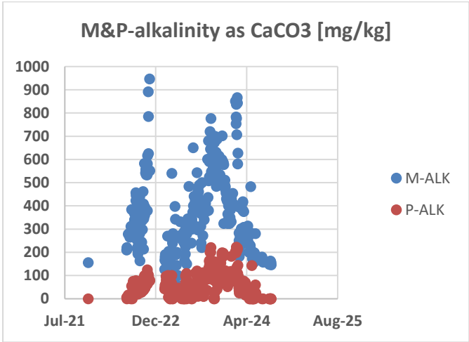
Figure 19: Dirty water dam recovery M&P alkalinity at Tutuka Power Station
