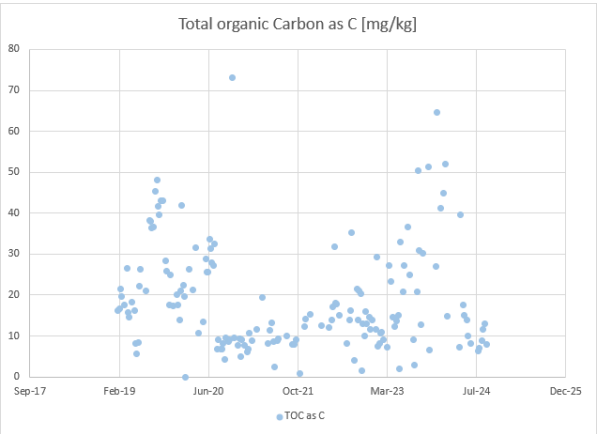
Figure 92: Tutuka Cooling water West total organic carbon
