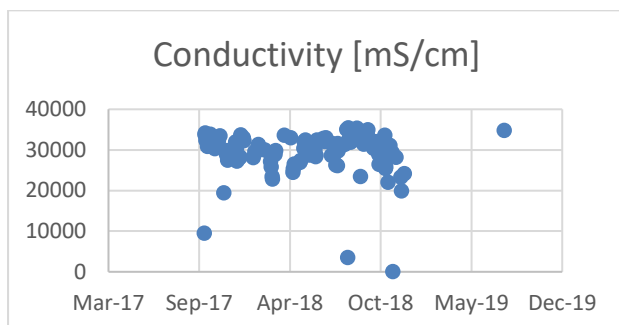
Figure 40: Tutuka SRO brine conductivity
