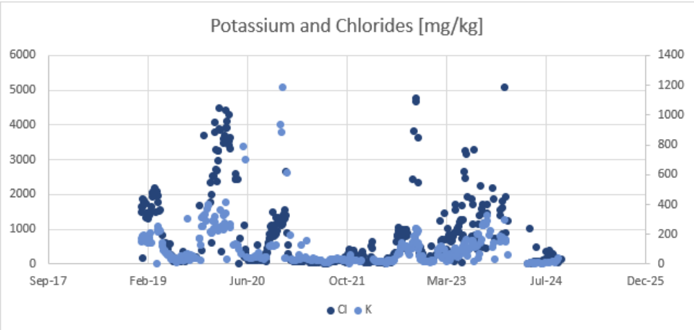
Figure 77: Tutuka Cooling water East Chlorides and Potassium
