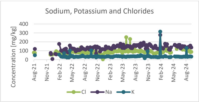
Figure 30: Duvha Ash Water Sodium, Chlorides and Potassium
