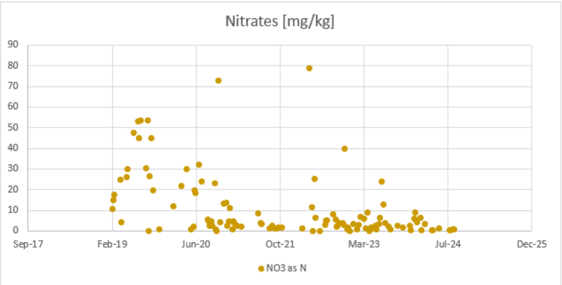
Figure 89: Tutuka Cooling water West Nitrates
