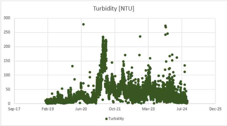
Figure 83: Tutuka Cooling water West turbidity
