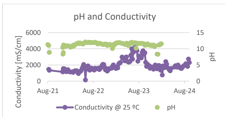
Figure 26: Duvha Ash Water pH and Conductivity
