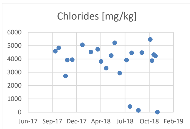
Figure 49: Tutuka SRO chlorides concentration
