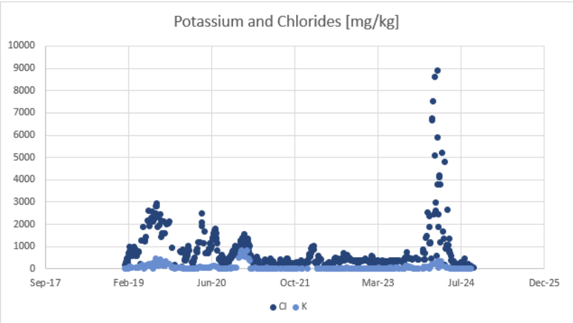
Figure 88: Tutuka Cooling water West Potassium and chlorides
