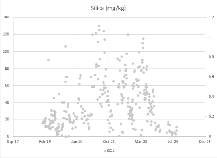
Figure 80: Tutuka Cooling water East Silicates
