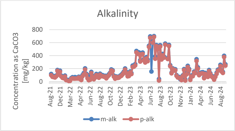
Figure 29: Duvha Ash Water Alkalinity
