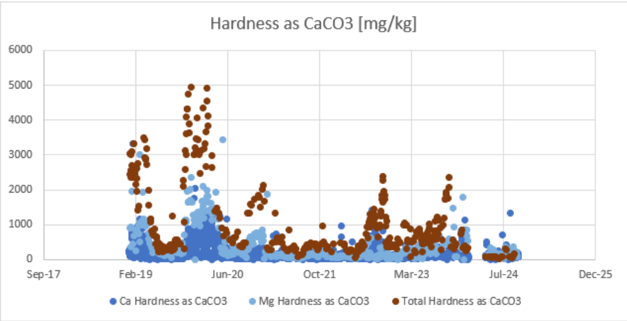
Figure 73: Tutuka Cooling water East Hardness
