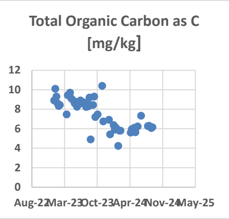
Figure 9: Raw water Total organic carbon
