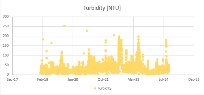
Figure 54: Kriel Cooling water South Turbidity
