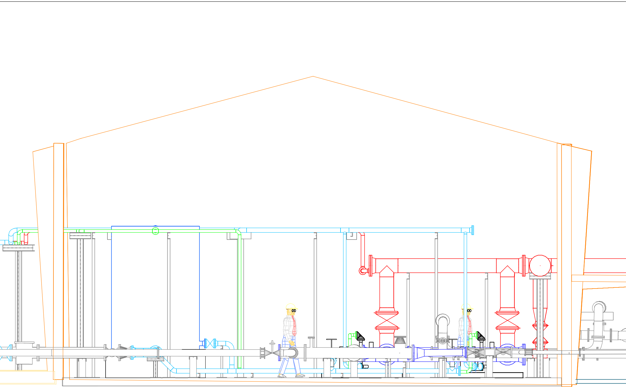
SECTION C-C PLAN VIEW ON 16684-D01 SCALE 1:50
