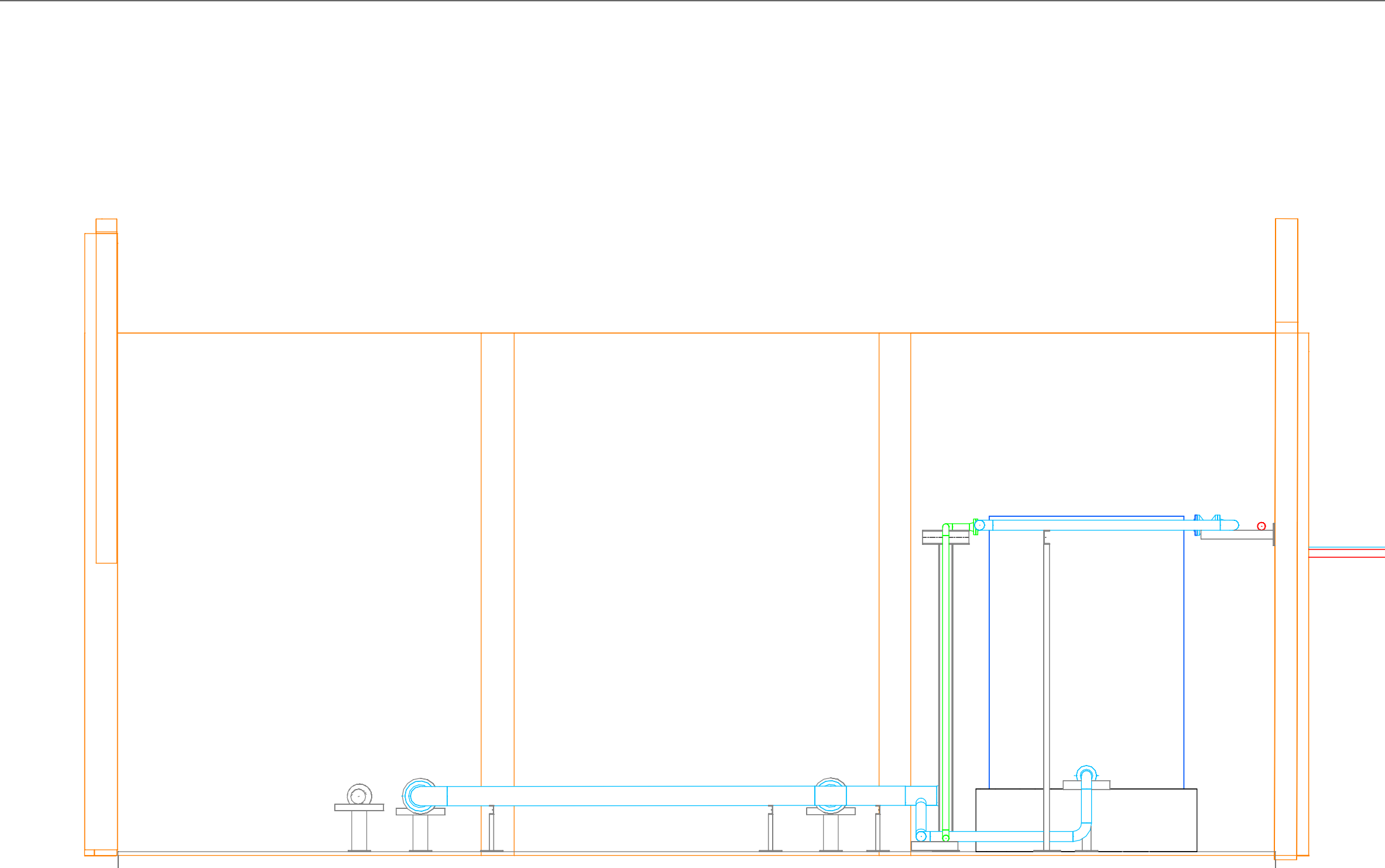
SECTION A-A PLAN VIEW ON 16684-D01 SCALE 1:50
