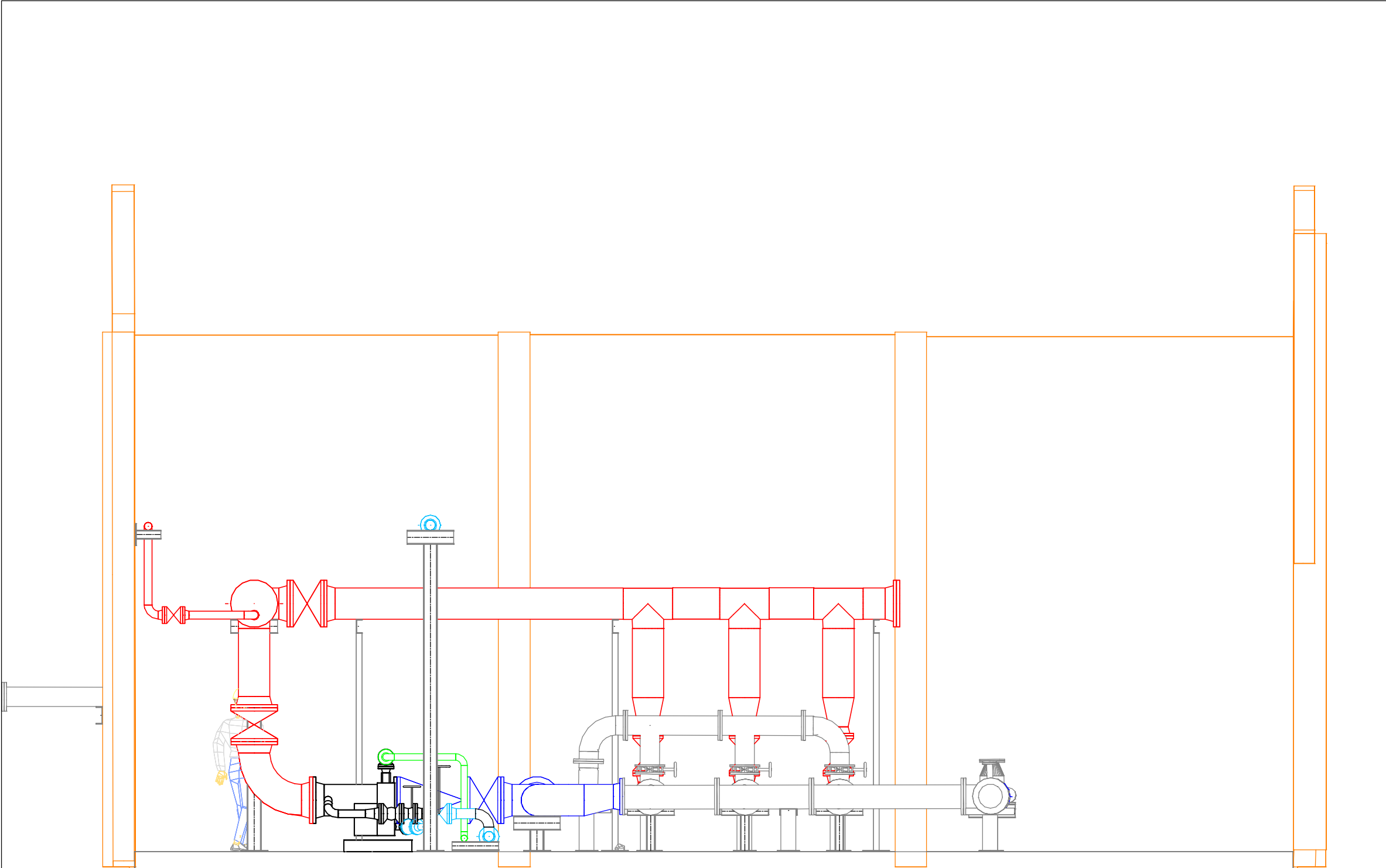
SECTION B-B PLAN VIEW ON 16684-D01 SCALE 1:50
