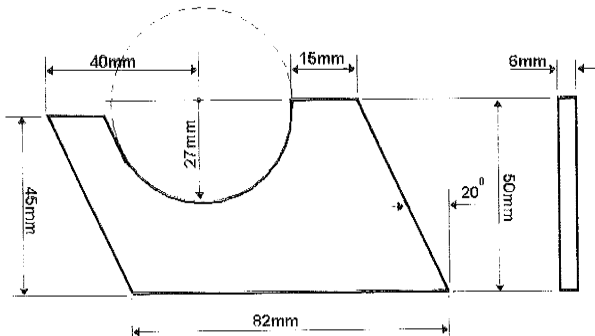
Retaining Bracket for 51mm = OD tube.
