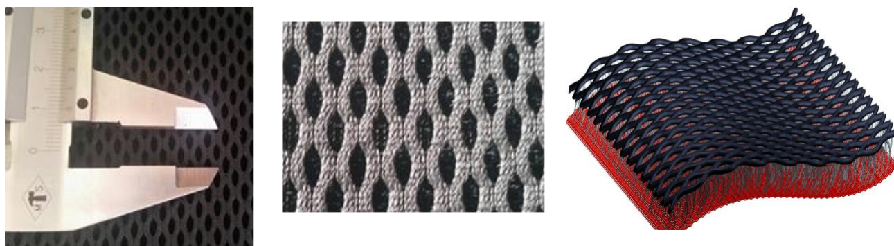
Figure 9 – Construction of spacer fabric
