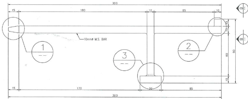
TYPICAL DETAIL OF METER TOOL
