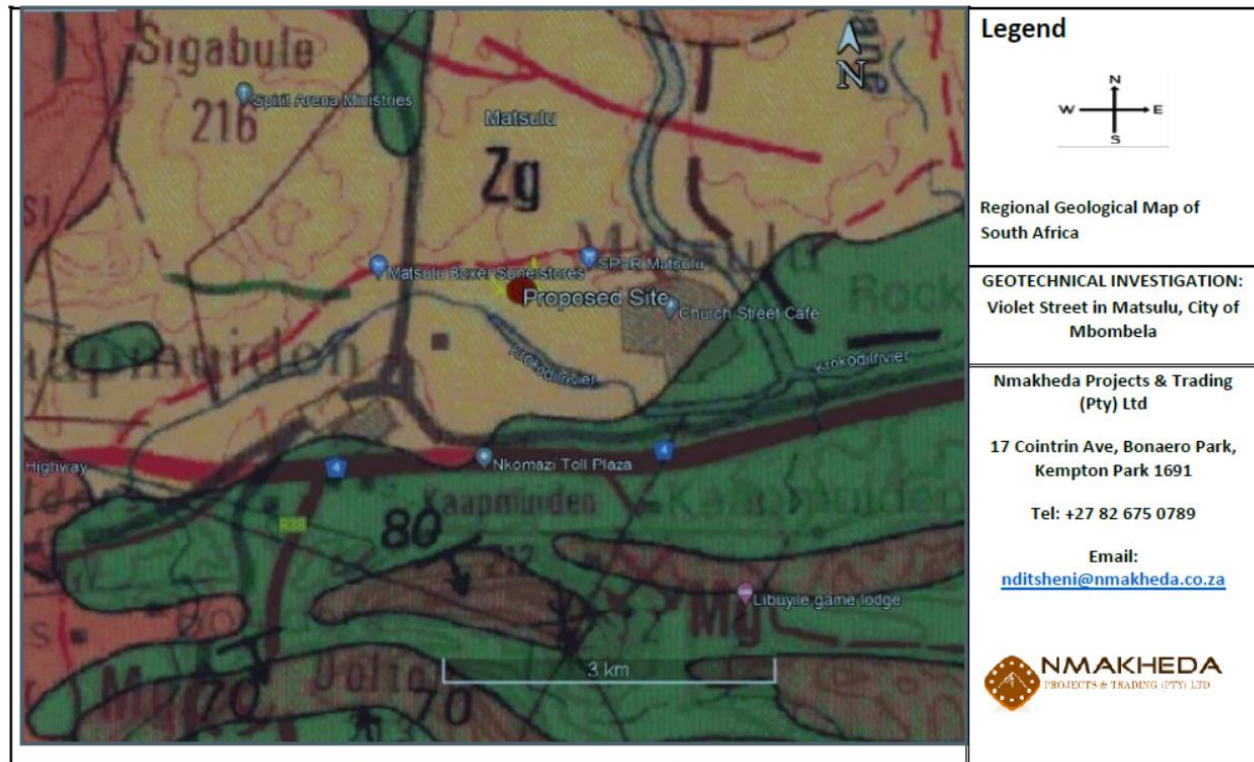
Figure 3: Extract from the 1:250 000 Geological Map (2530) Baberton.
