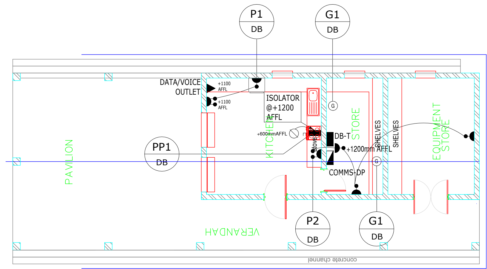
Plan – TUCK SHOP
