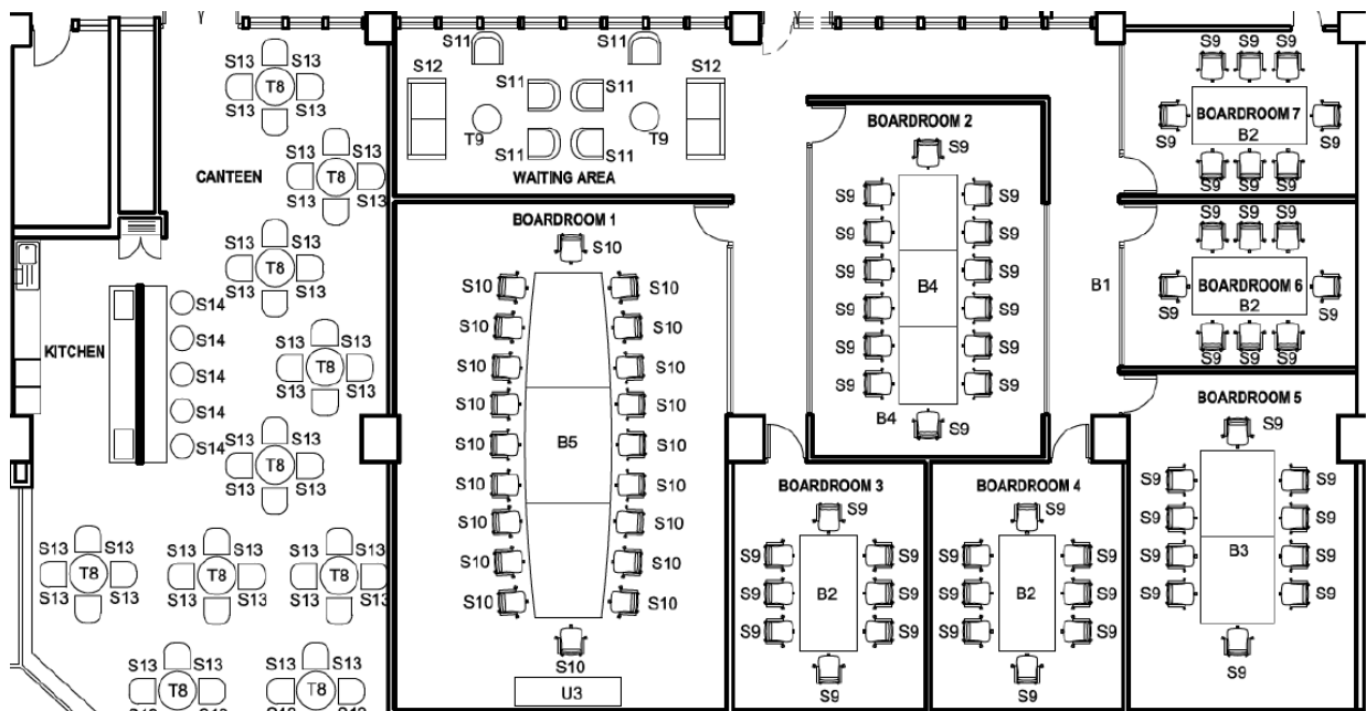
Figure 1, Floor layout
