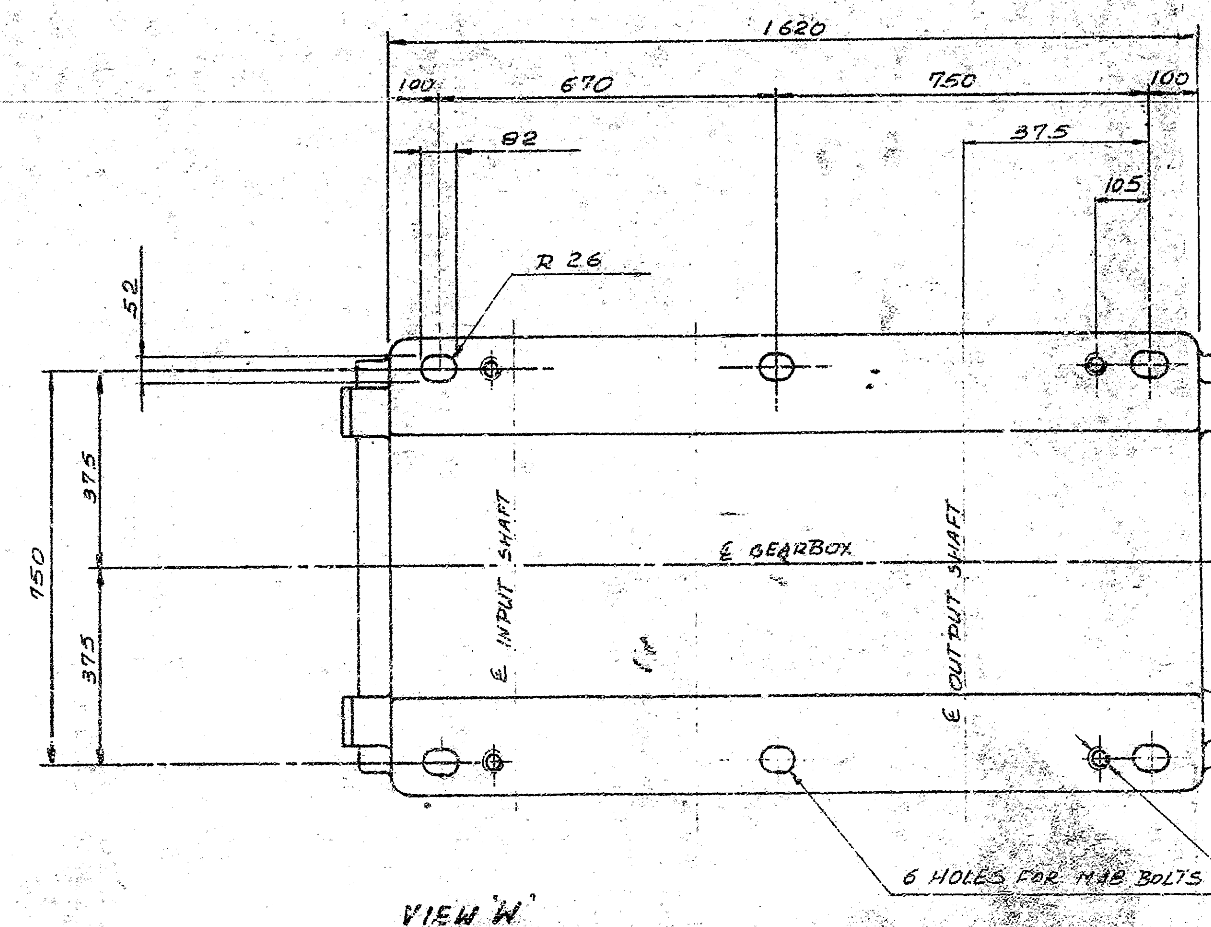
VIEW 'W' DETAIL OF BASE LOOKING AT DIRECTION ON VIEW 'W'
