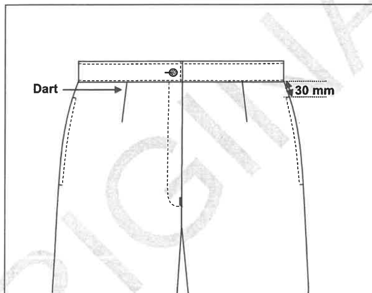
Figure 3 – Plain fronts with darts
