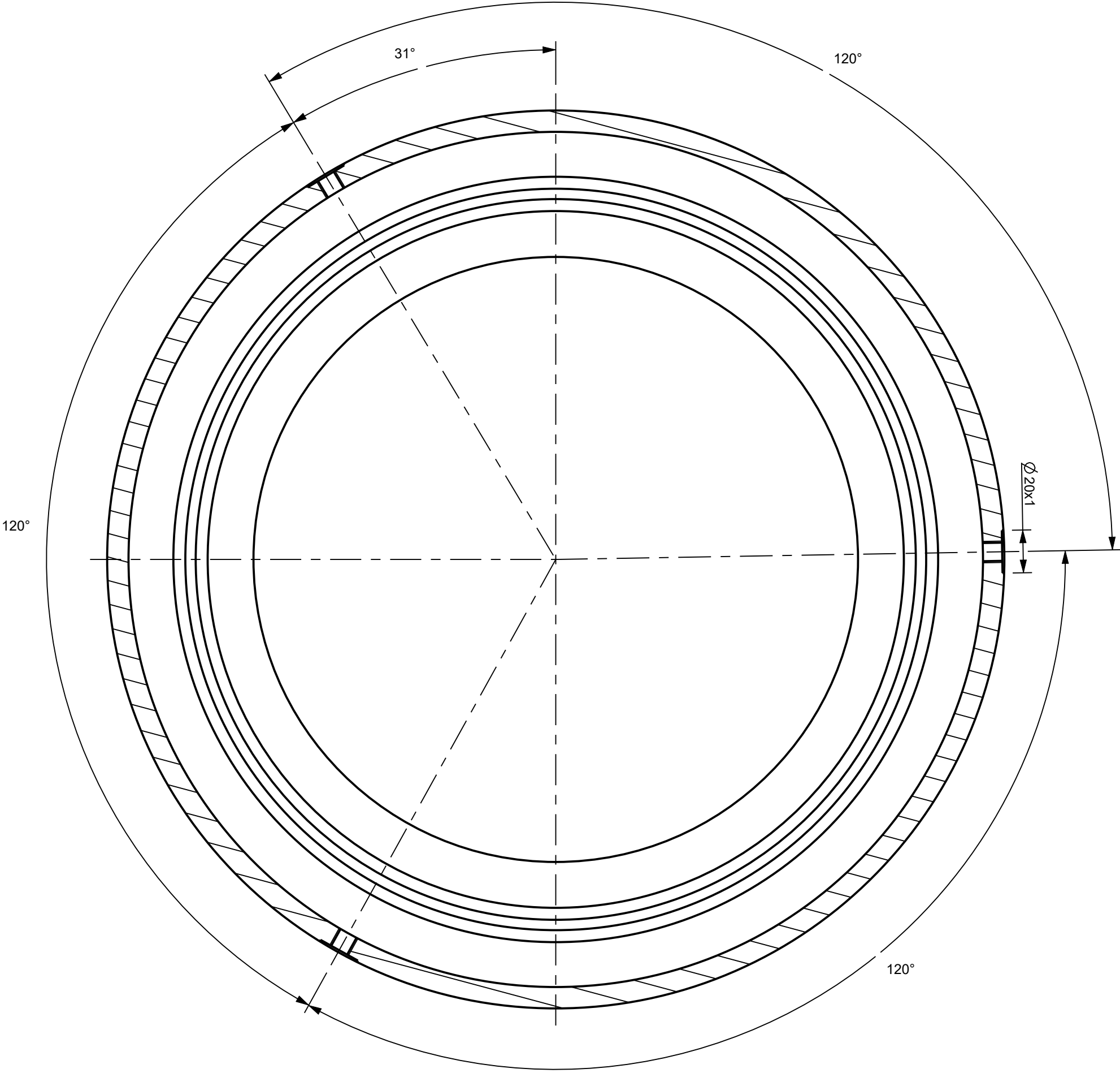
SECTION C-C
