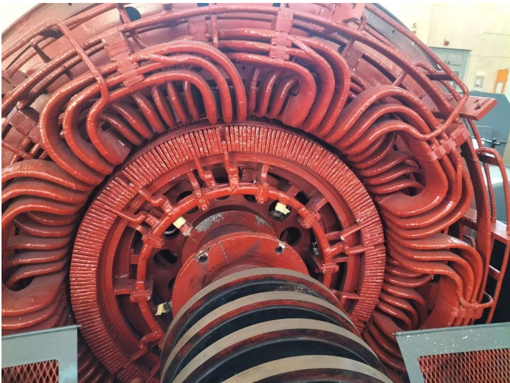
Stator and rotor
