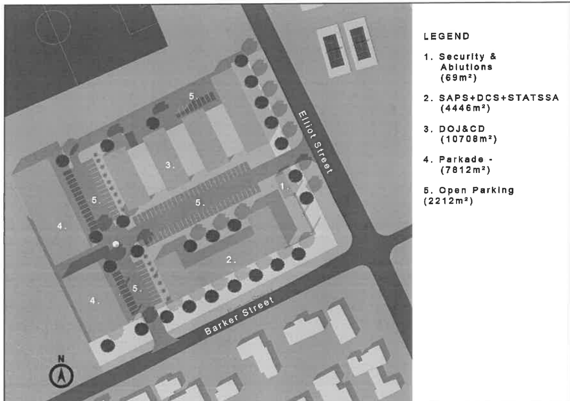
Precinct Development Plan
