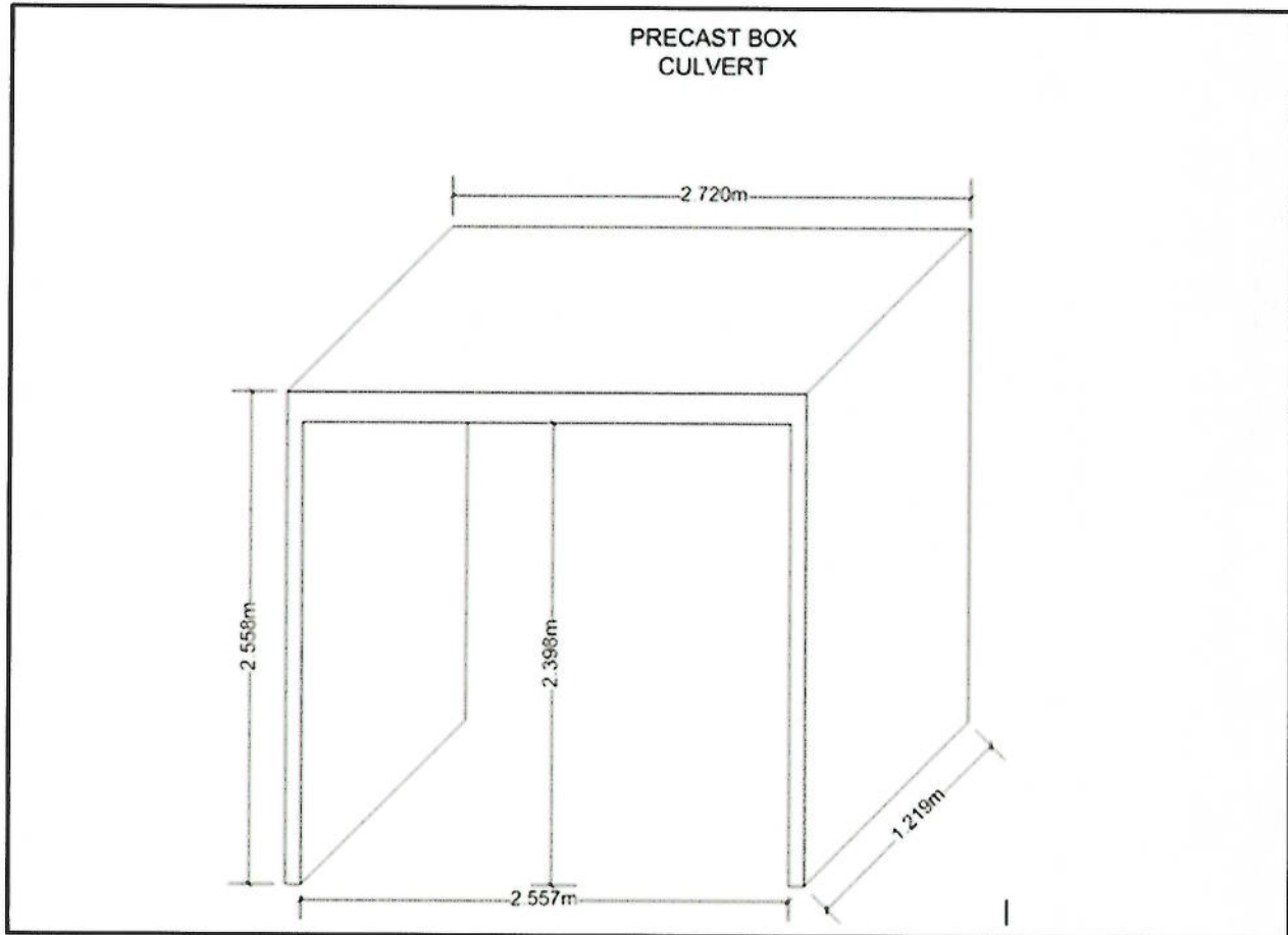
Culvert Dimensional Layout
