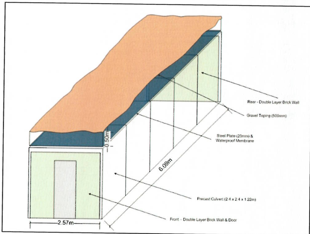
Office Cubicle Dimensions
