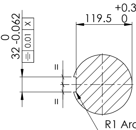
SECTION I-I
