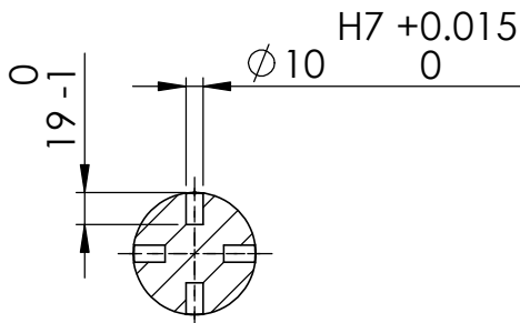
SECTION M-M Use Flat Bottom Milling Cutter
