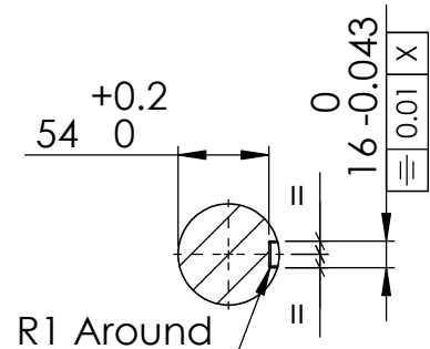
SECTION L-L
