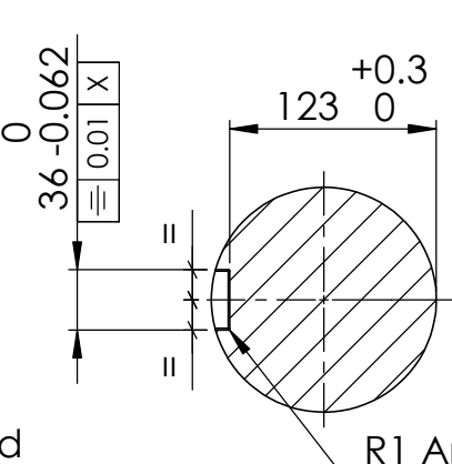
SECTION J-J
