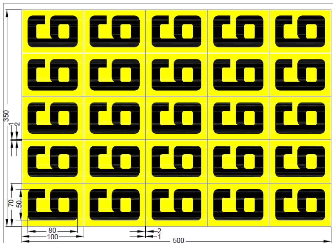
Figure 7 – Pole number "6"
