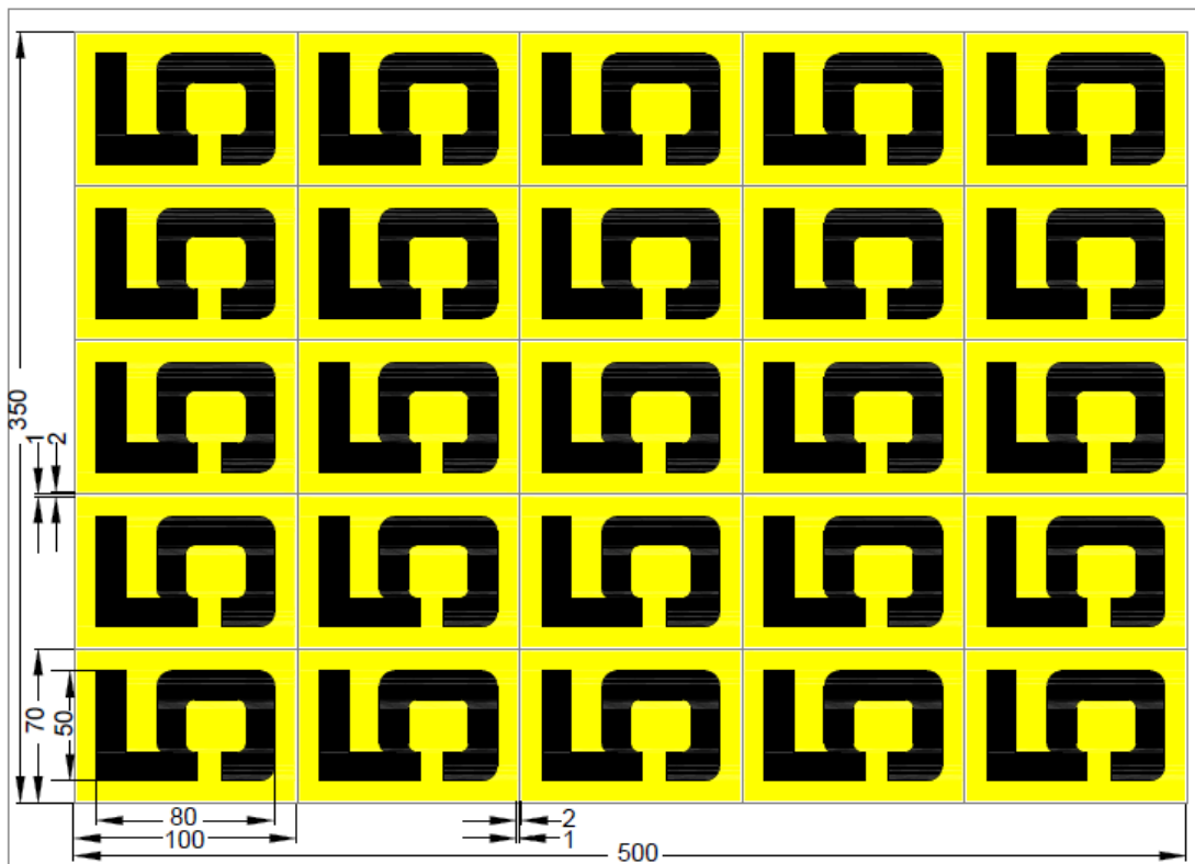
Figure 6 – Pole number "5"
