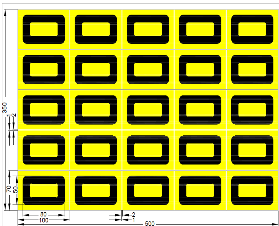
Figure 1 – Pole number "0"
