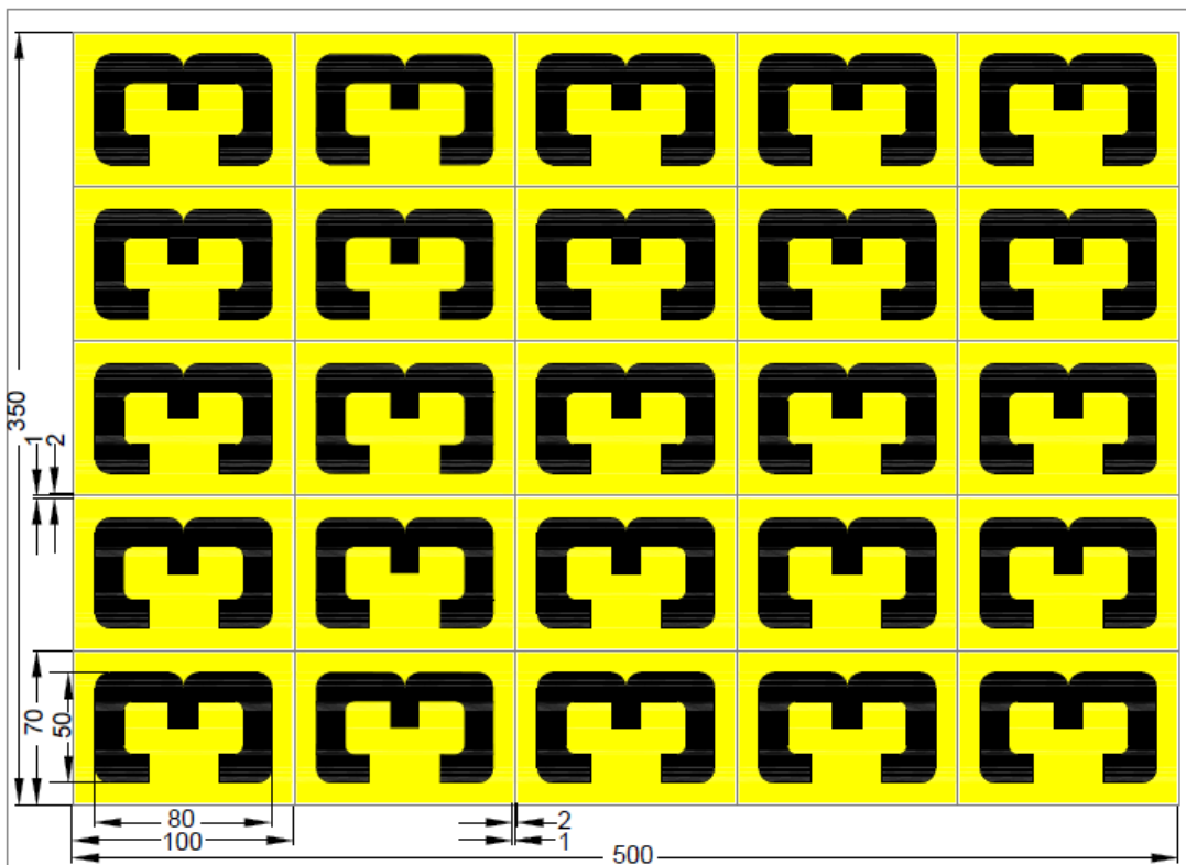
Figure 4 – Pole number "3"
