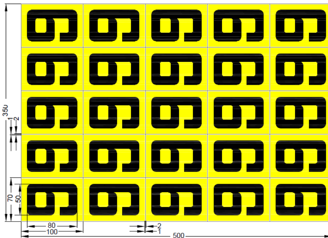
Figure 10 – Pole number "9"
