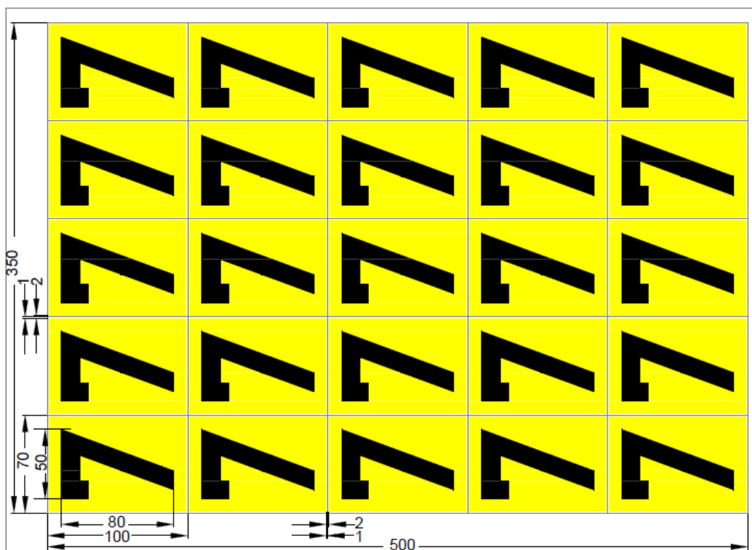
Figure 8 – Pole number "7"
