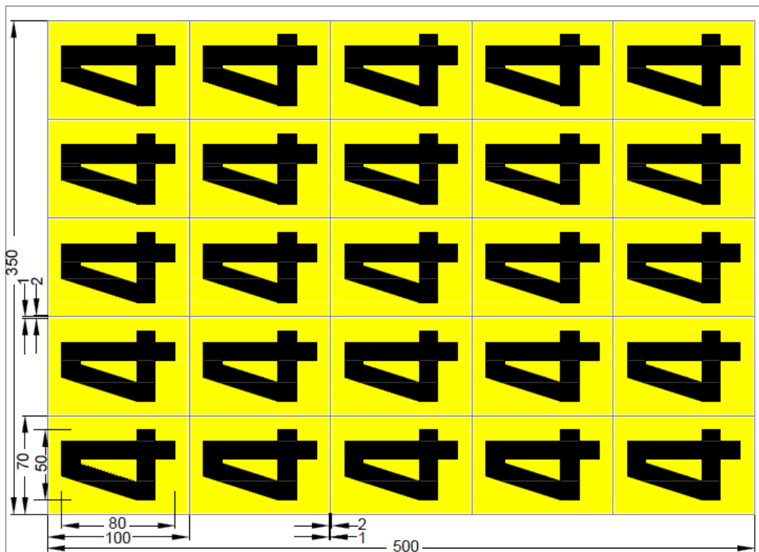
Figure 5 – Pole number "4"
