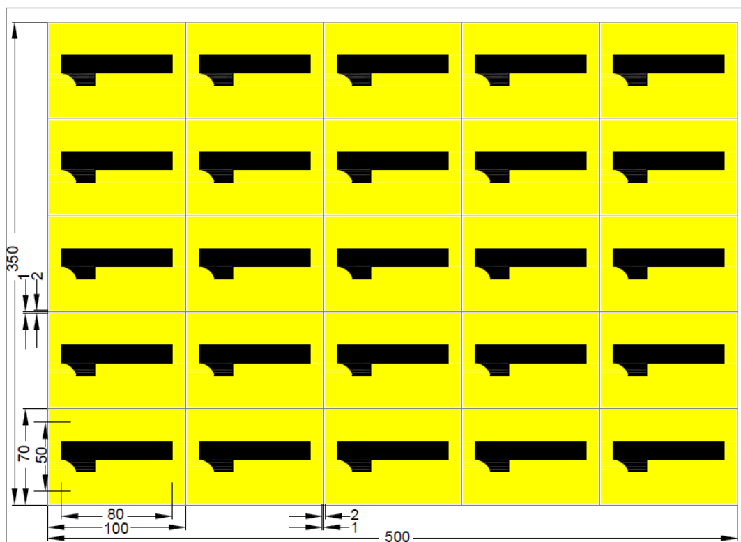
Figure 2 – Pole number "1"
