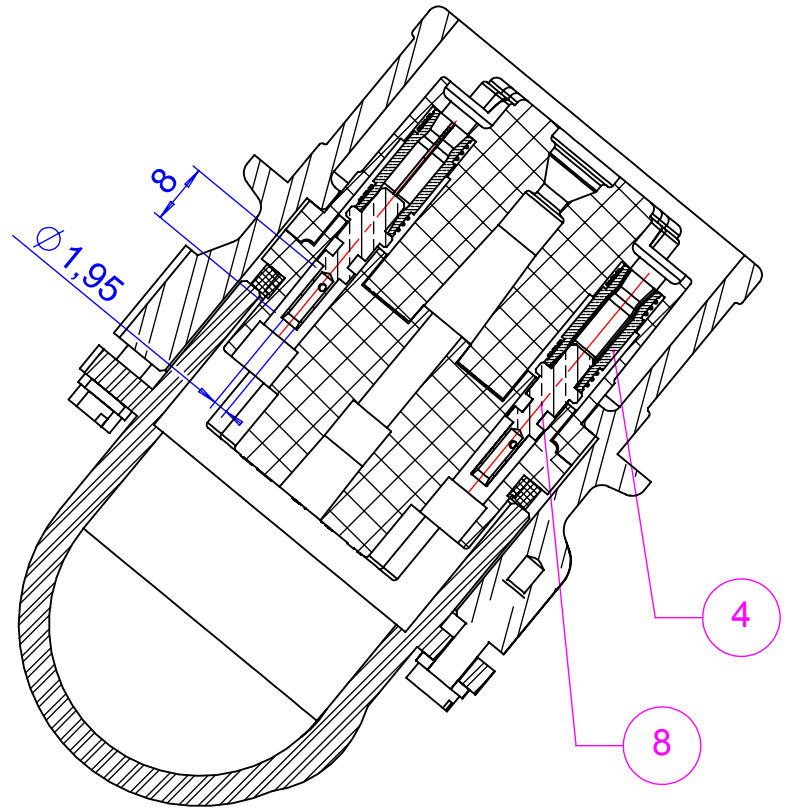
COUPE B-B (view of contacts Ø4 - 0.6 to 1.82 mm²)
