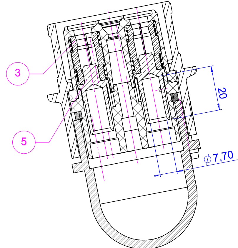
COUPE A-A (view of contacts Ø7 - 25 mm²)
