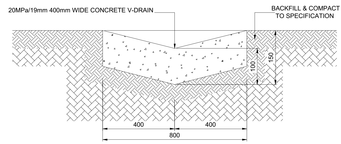
SECTION B - B CONCRETE CHANNEL SCALE 1:5
