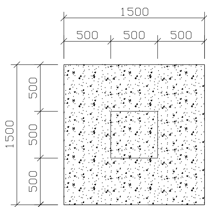
FOUNDATION LAYOUT
