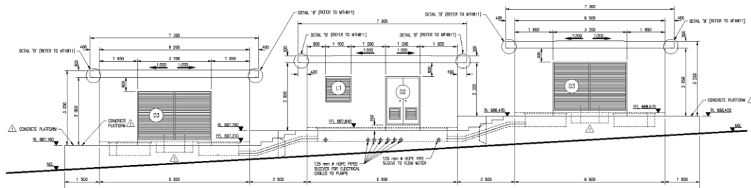
SOUTH ELEVATION SCALE 1:50
