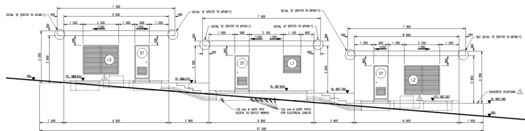
NORTH ELEVATION SCALE 1:50
