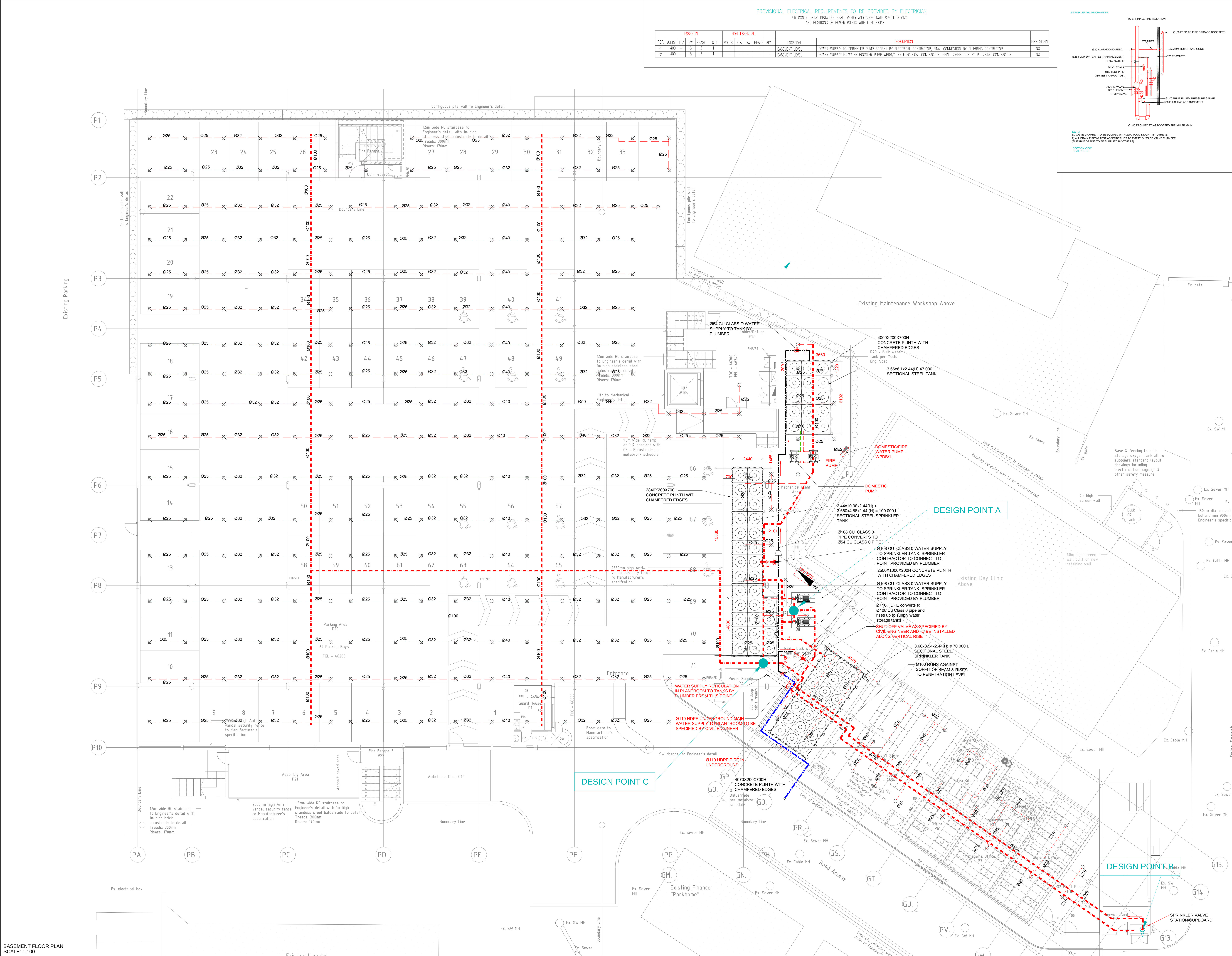
BASEMENT FLOOR PLAN SCALE: 1:100
