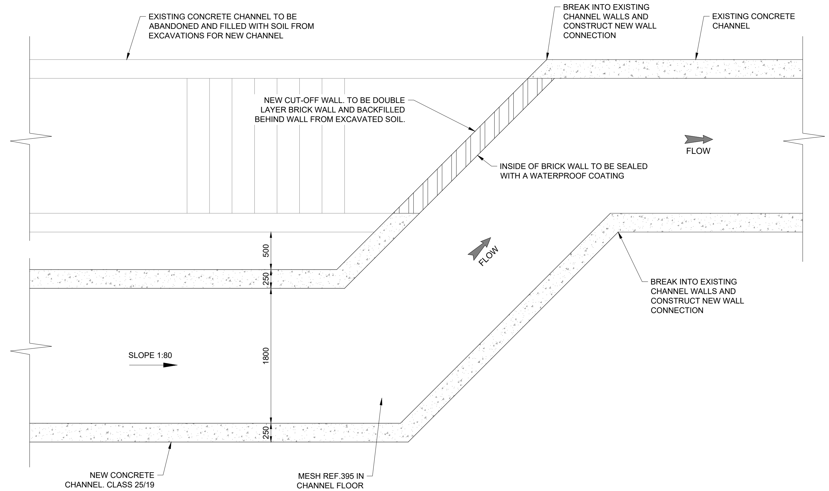
CHANNEL END DETAIL SCALE 1:30
