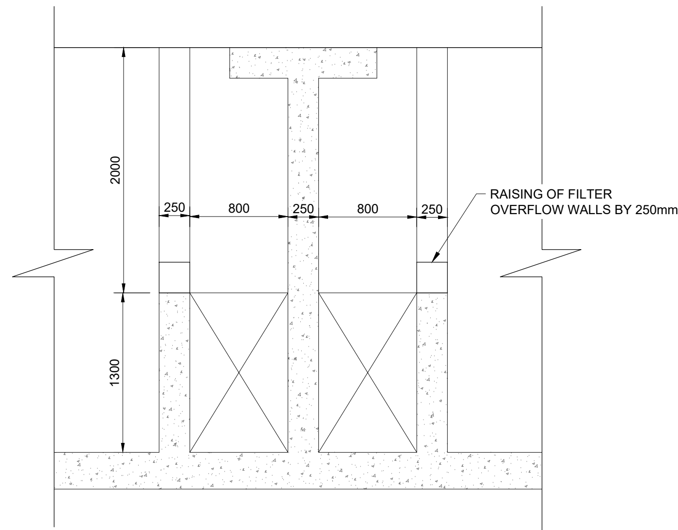
SECTION OF FILTER WALLS SCALE 1:30
