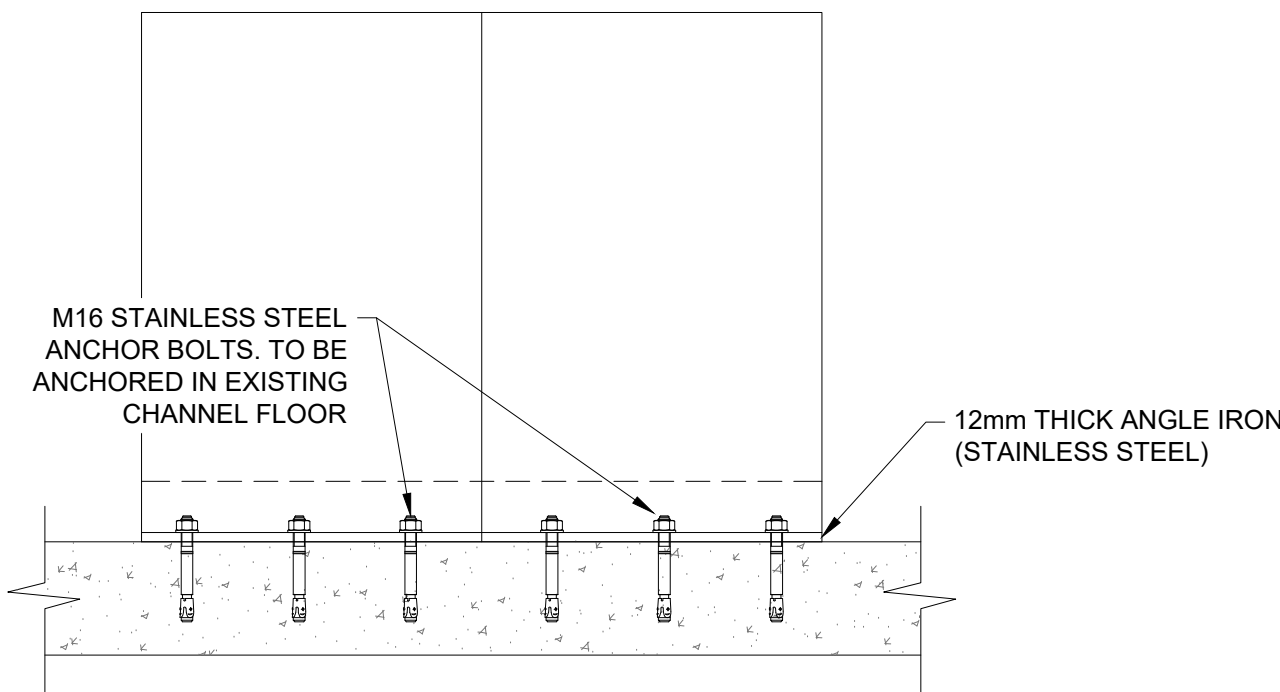
VEE BAFFLE ANCHORS FRONT VIEW SCALE 1:10
