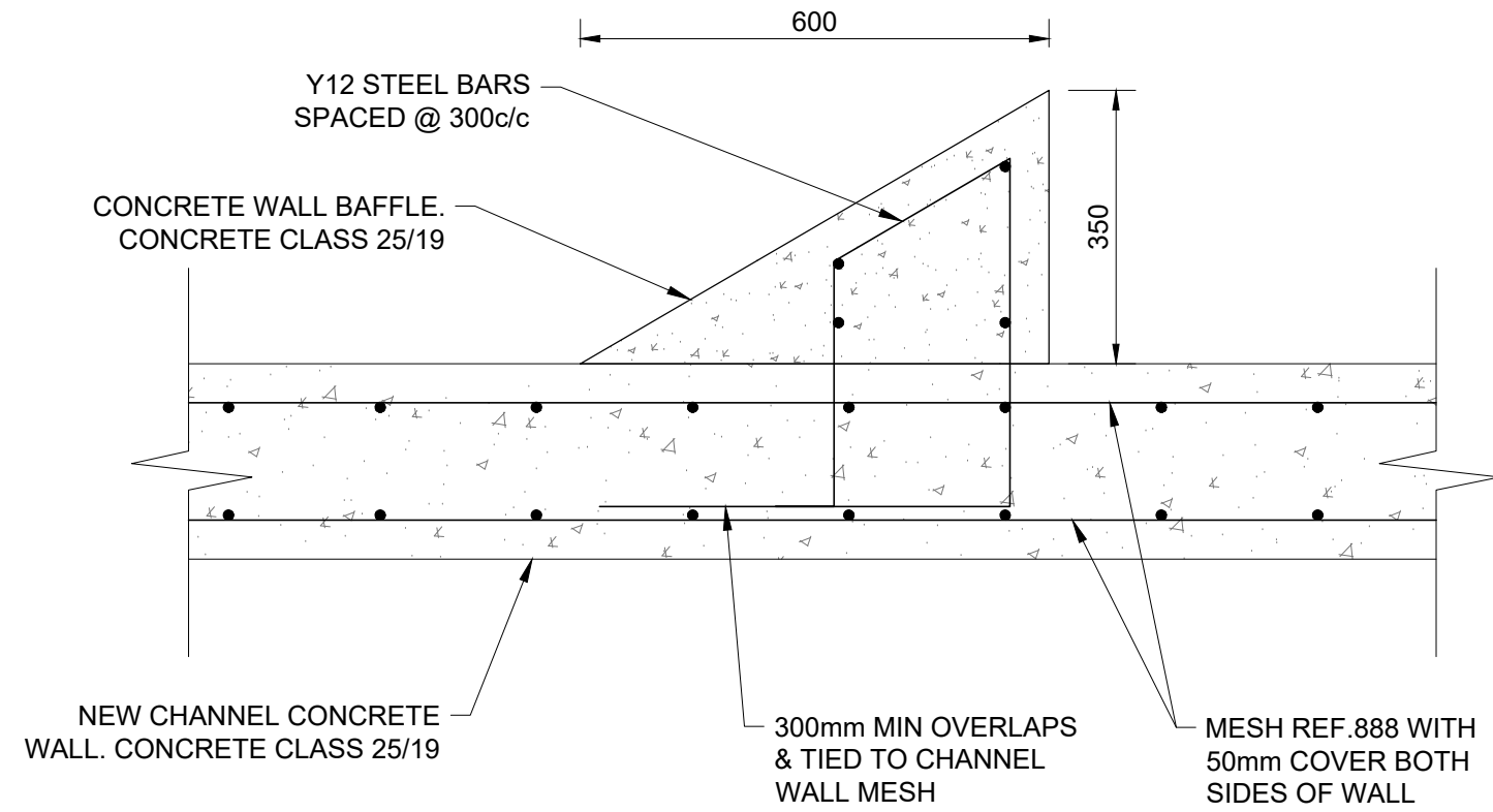
CONCRETE WALL BAFFLE PLAN VIEW SCALE 1:10
