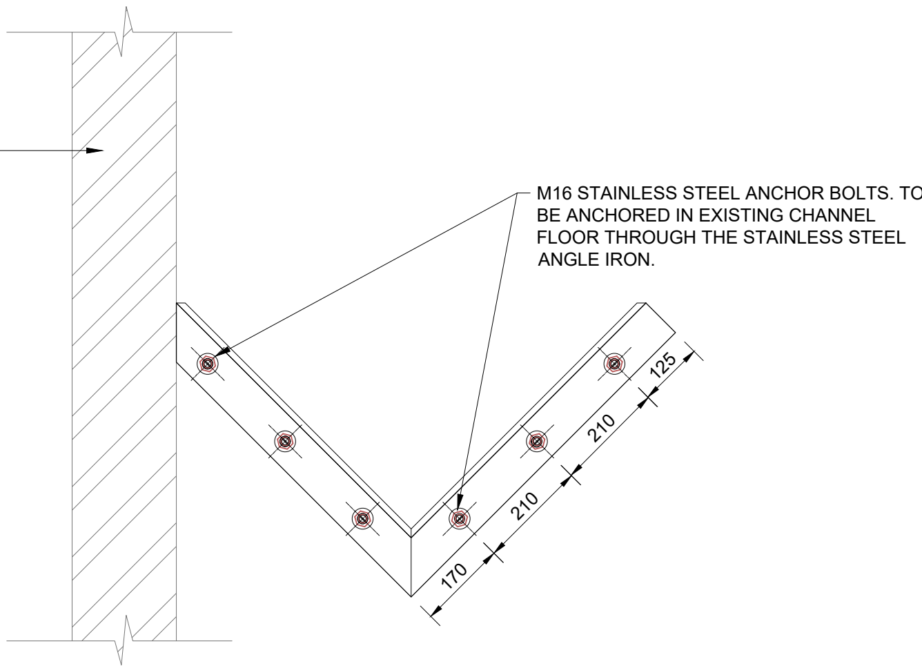
VEE BAFFLE ANCHORS PLAN VIEW SCALE 1:10
