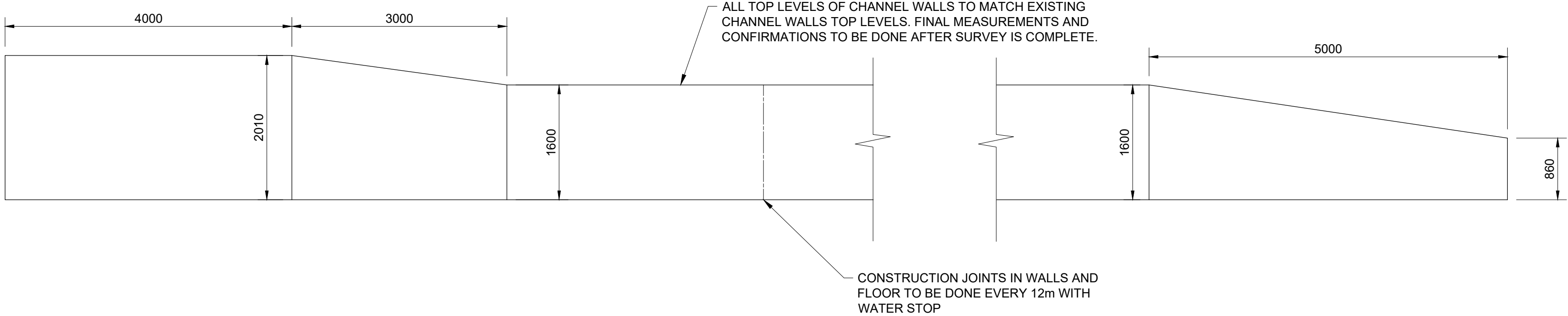
SIDE ELEVATION OF FLOCCULATION CHANNEL SCALE 1:50
