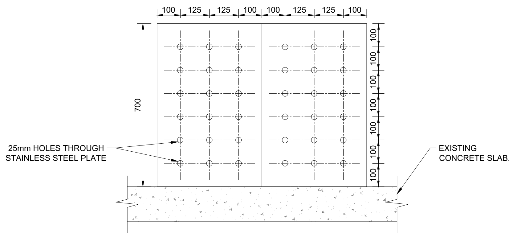
VEE BAFFLE PLATES SECTION C-C SCALE 1:10
