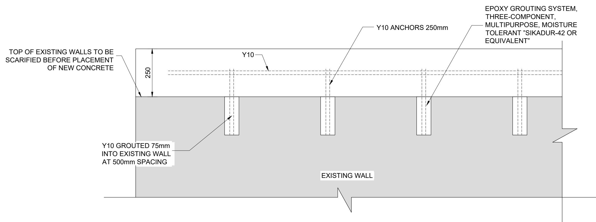
TYPICAL RAISING OF WALLS ON SAND FILTERS SCALE 1:10
