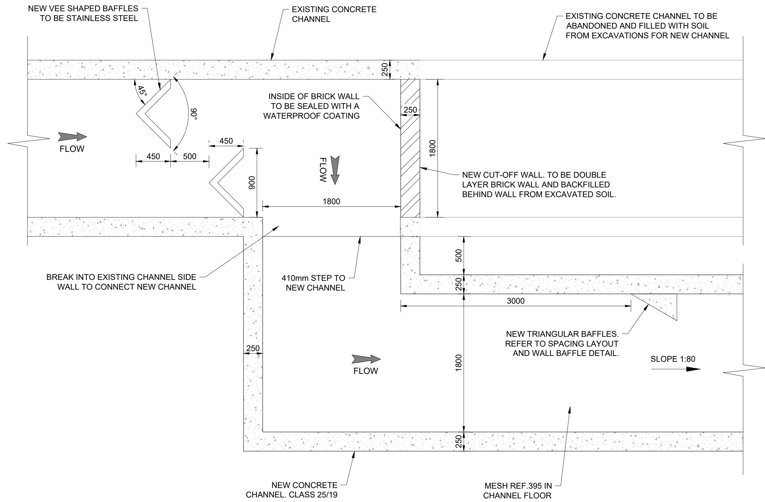
CHANNEL START DETAIL SCALE 1:30
