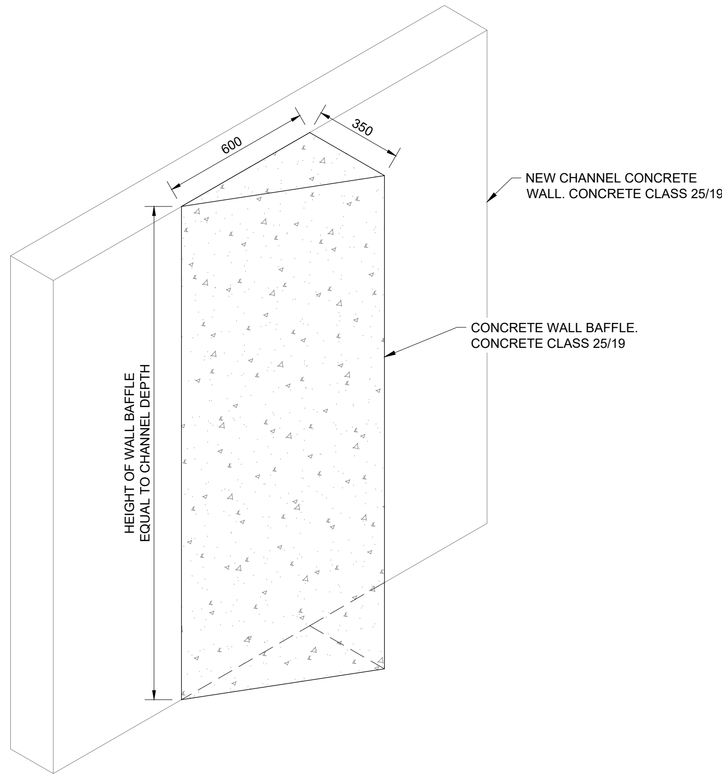
CONCRETE WALL BAFFLE ISOMETRIC VIEW SCALE 1:15
