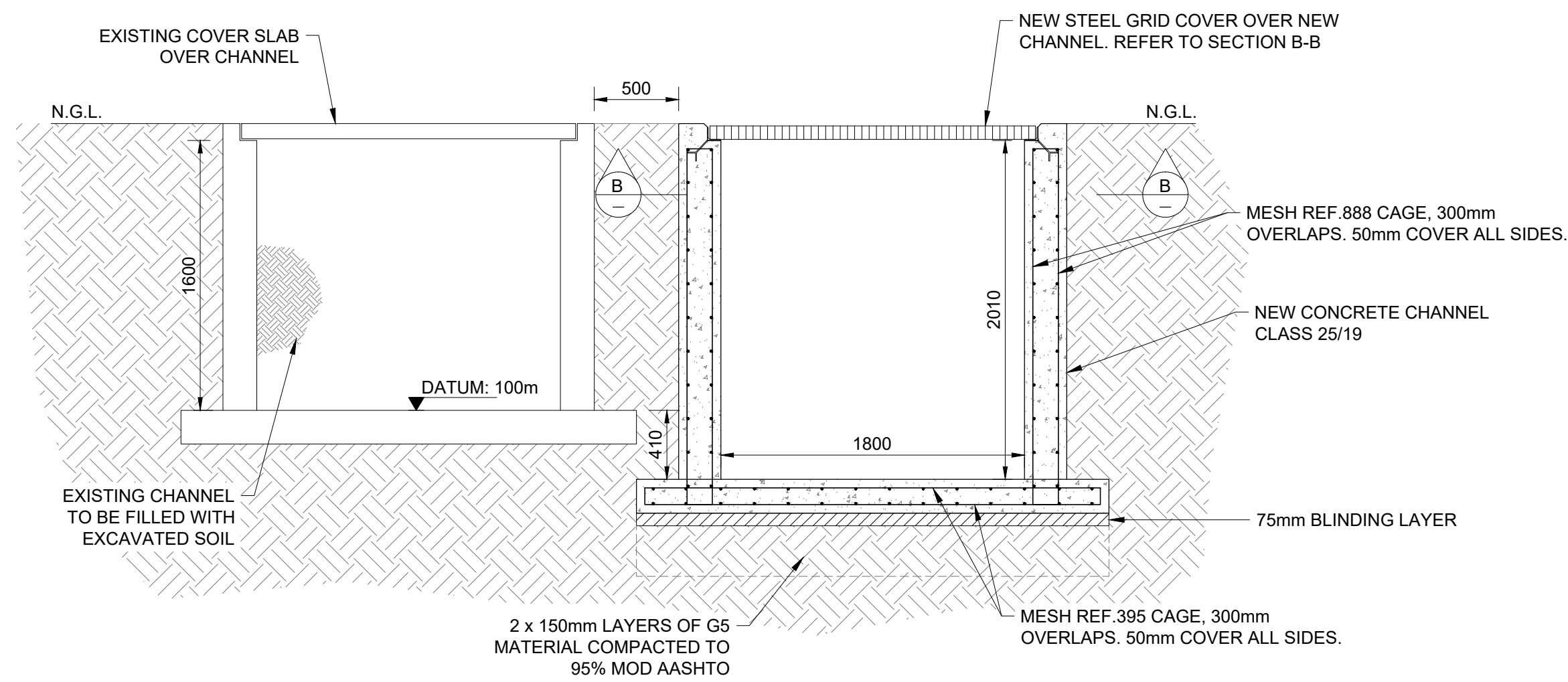
CHANNEL CROSS-SECTION SECTION A-A SCALE 1:30
