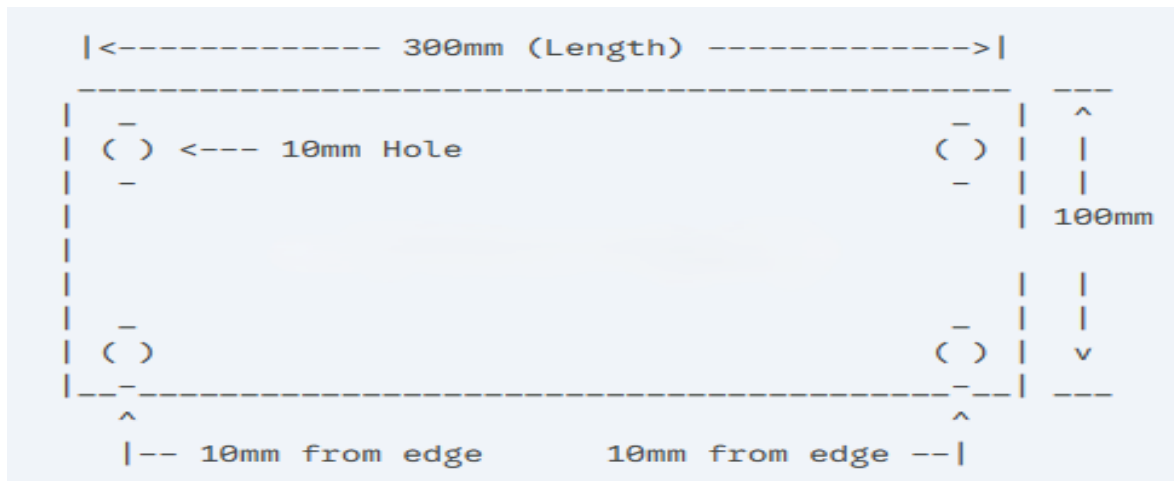
Figure 2: Numbering Plate Template
