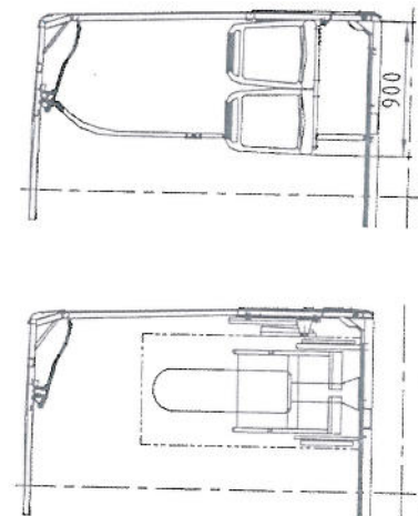
Cross-section at wheelchair space
