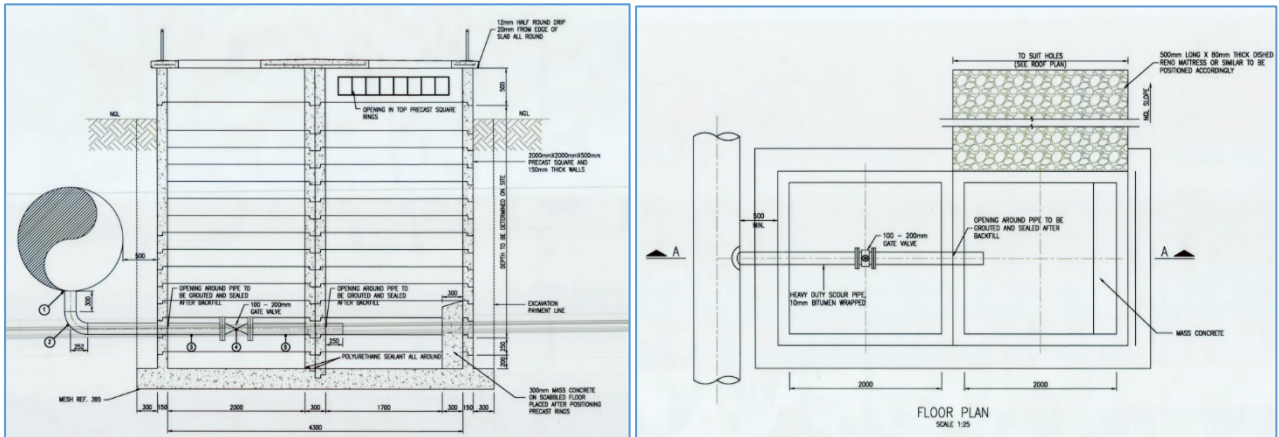
Figure 5 and 6: Typical scour valve chamber and the associated pipe fittings (design guidelines)
