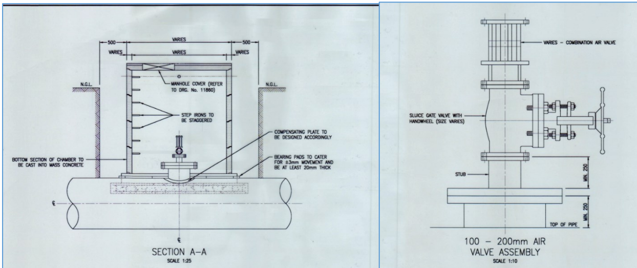
Figure 3 and 4: Typical in-line air valve chamber with isolator valve and the associated pipe fittings (design guidelines)
