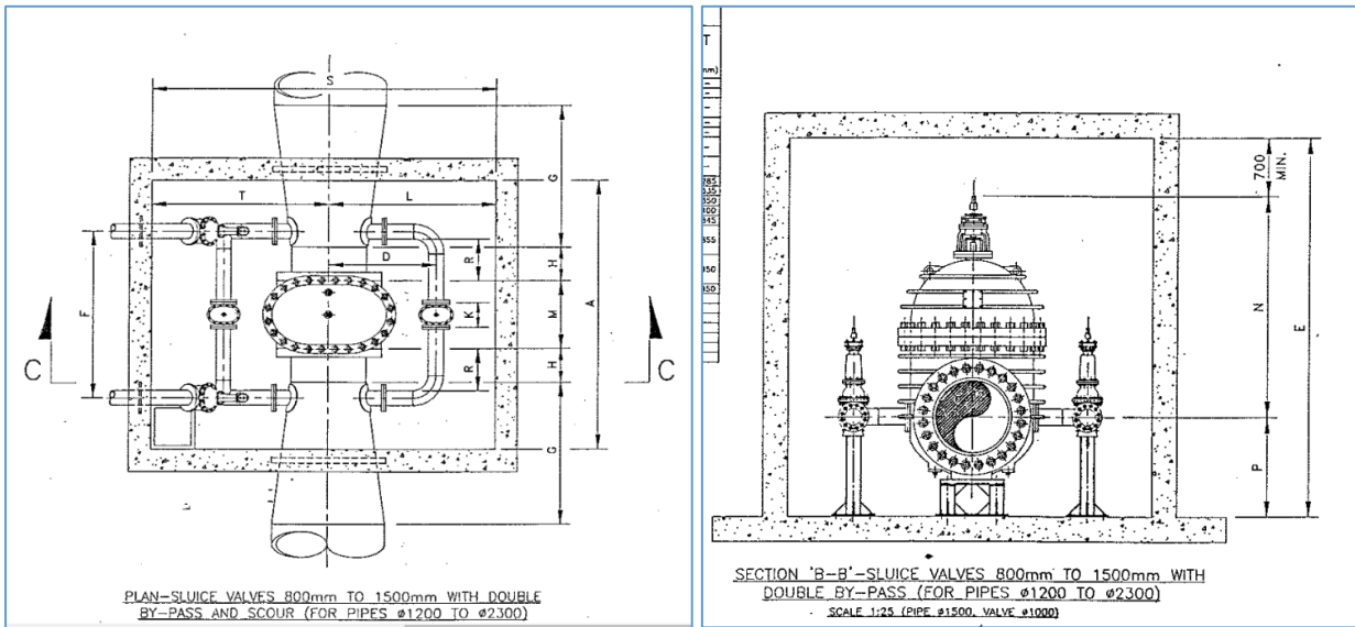
Figure 1 and 2: Typical in-line isolating valve chamber with by-pass valves and the associated pipe fittings (design guidelines)
