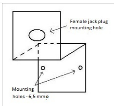
Figure 2 – Mounting bracket for EFI jack plug
