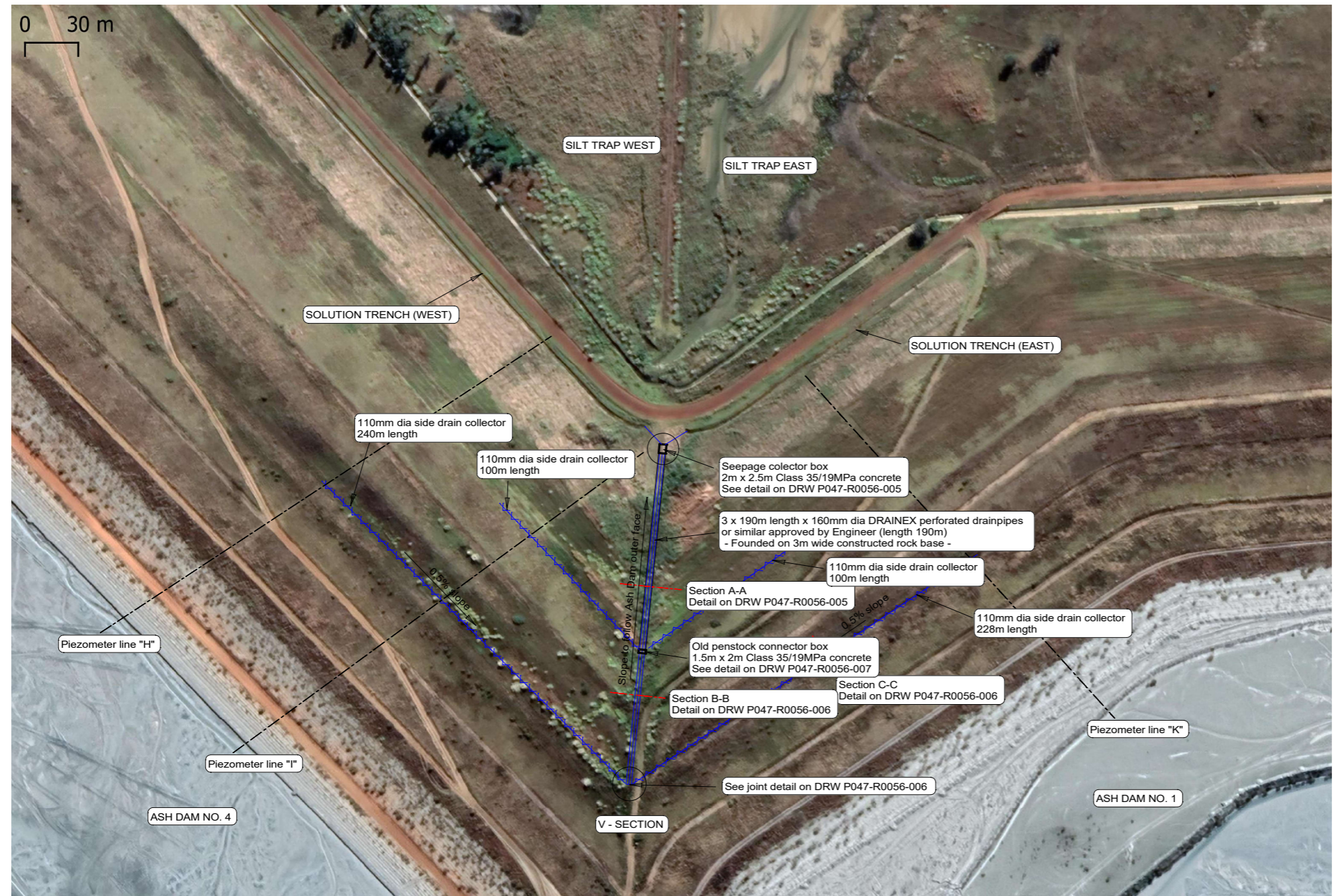
PLAN VIEW OF ADDITIONAL PIPE DRAINS INSTALLATION - SCALE 1:2250 (A3) -
