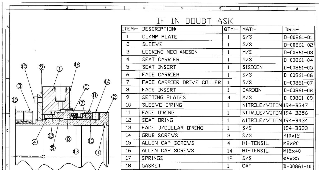
Mechanical seal drawing
