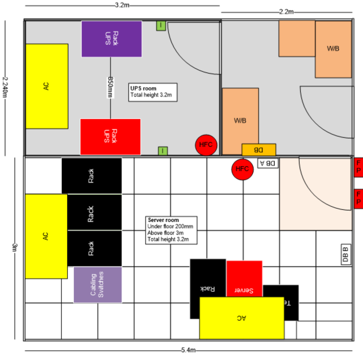
FLOOR PLAN OF SERVER ROOM
