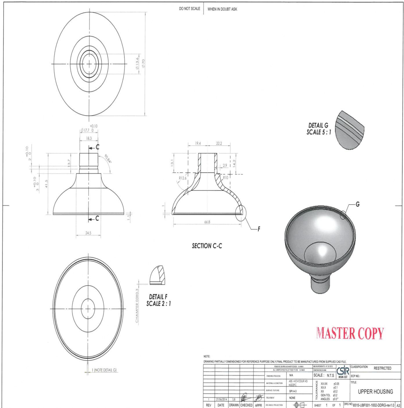
Figure 3: Technical drawing of the part corresponding to the upper mould
