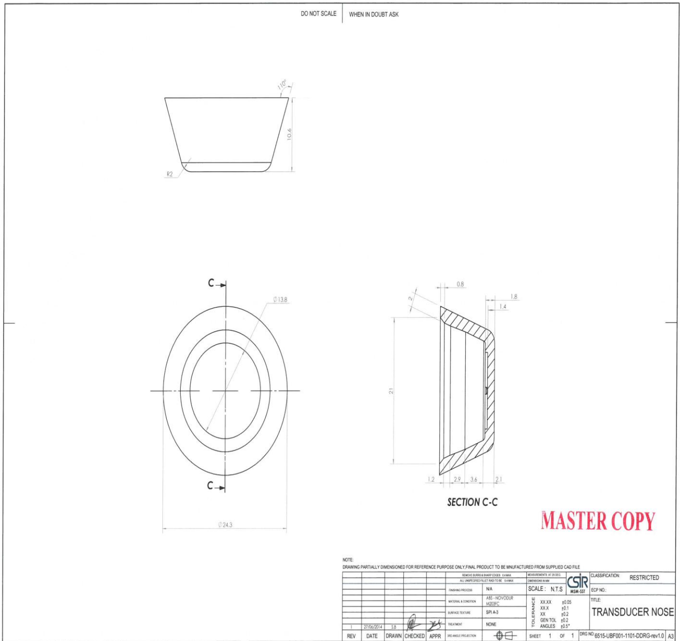
Fig 6: Technical drawing of the part corresponding to the Transducer Nose mould
