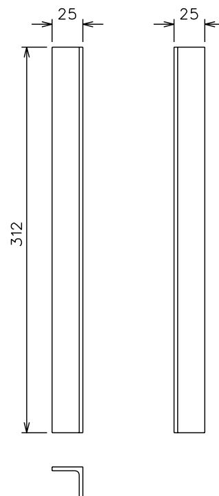
ITEM 3 - CROSSMEMBER STIFFNER 25x25x3x312 lg. EQUAL ANGLE (1 OFF) (SCALE 3:1)
