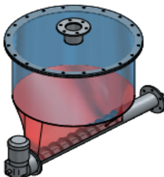
Figure 3 : Feed-hopper and screw-feeder assembly (To be used for information purpose)
