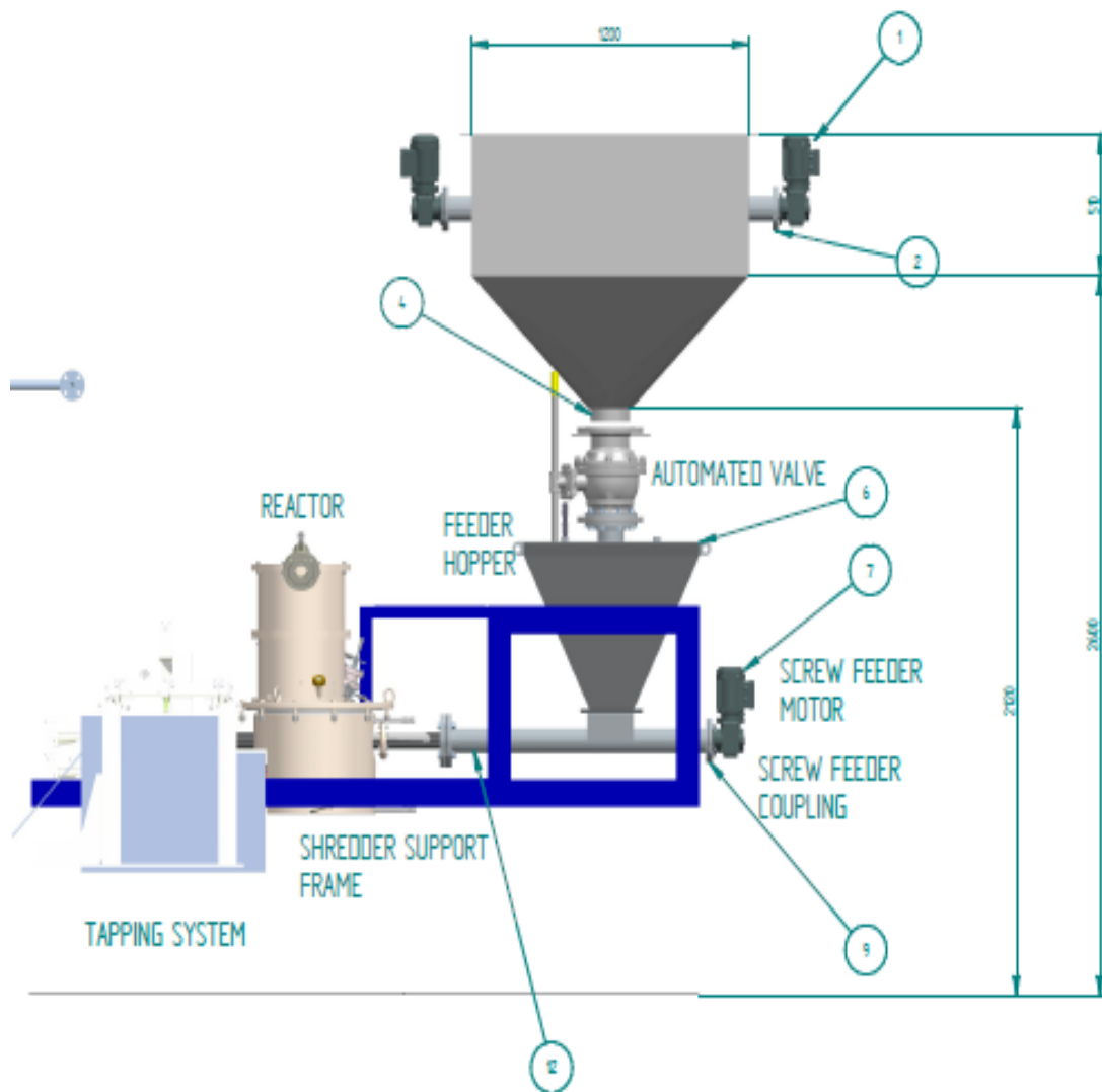
Figure 1 A : Shredder, feed-hopper and screw-feeder 2D sketch (To be used for quotation purpose)
