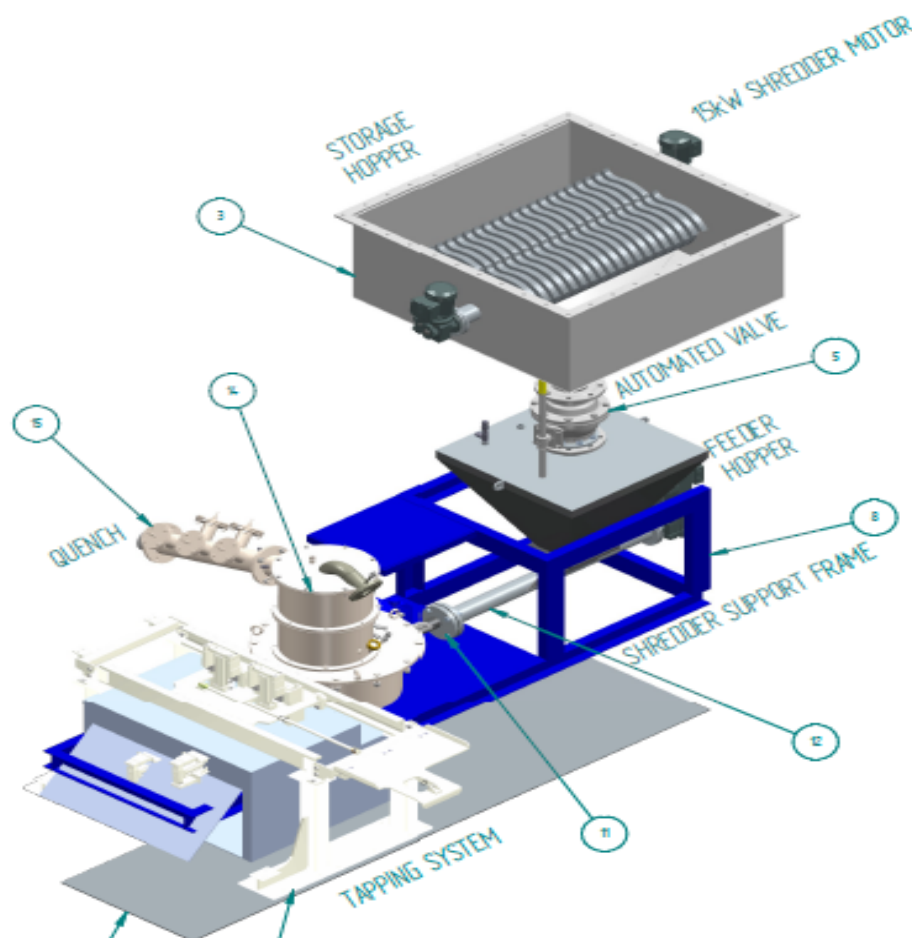
Figure 1 B: Shredder, feed-hopper and screw-feeder 3D snapshot (To be used for quotation purpose)
