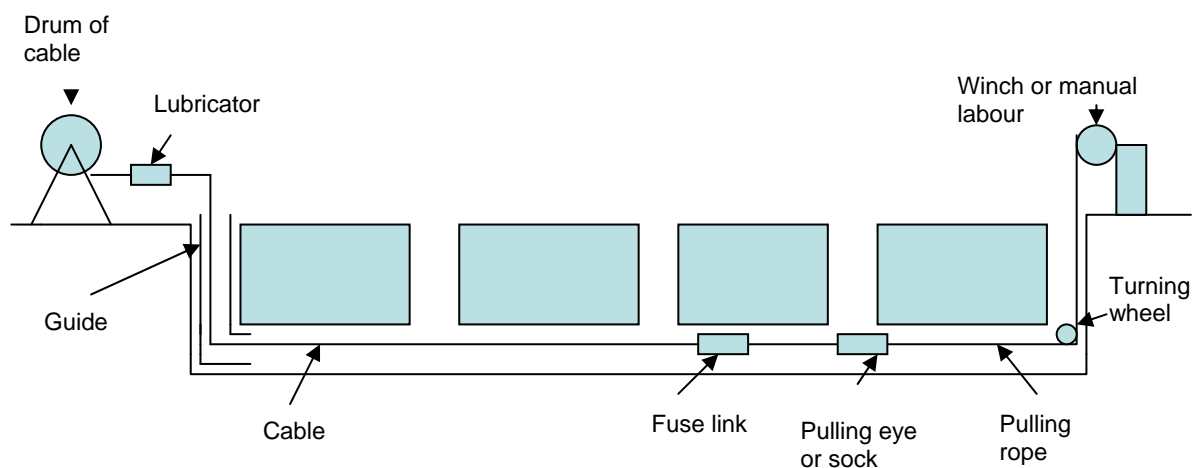
Figure 3 — Underground cable installation in ducts by winching
