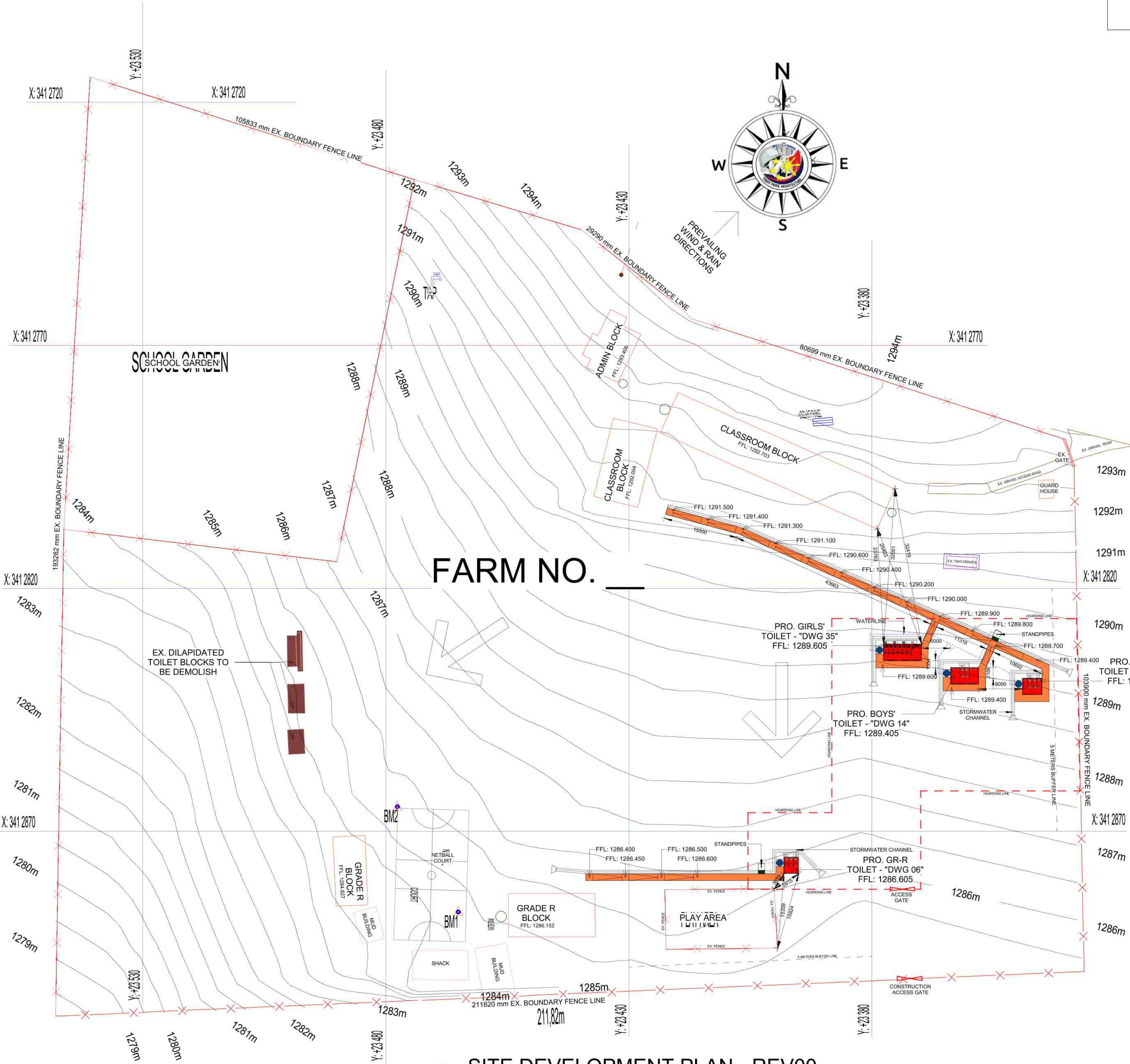
1 SITE DEVELOPMENT PLAN - REV00 1 : 500
