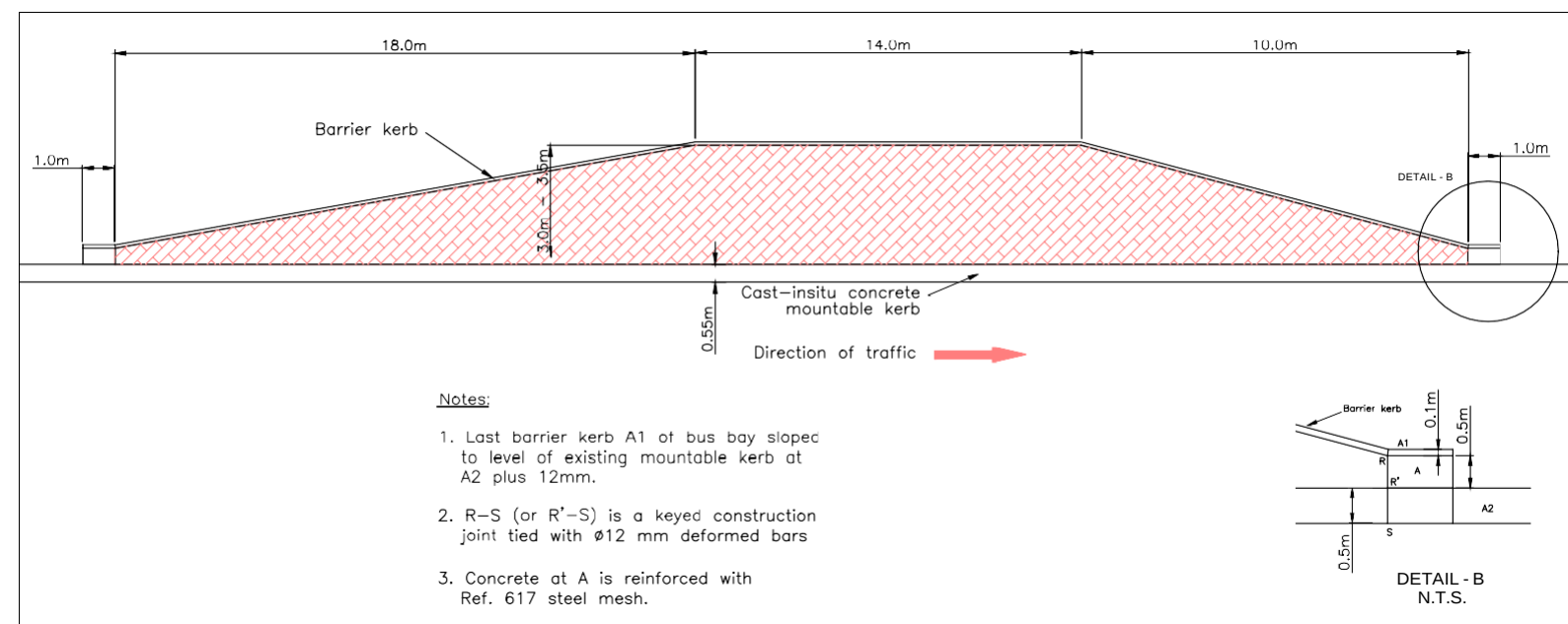
GEOMETRICAL LAYOUT OF BUS BAY FOR SINGLE BUS - USING CAST-IN SITU MOUNTABLE KERB SCALE - 1: 100
