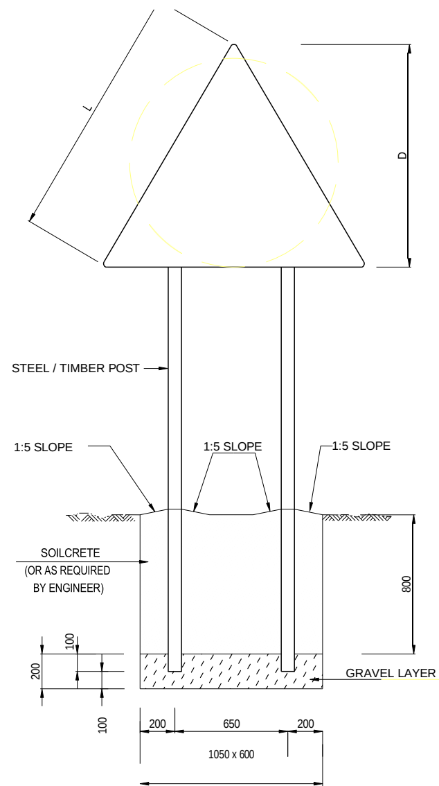
FOUNDATION DETAIL
