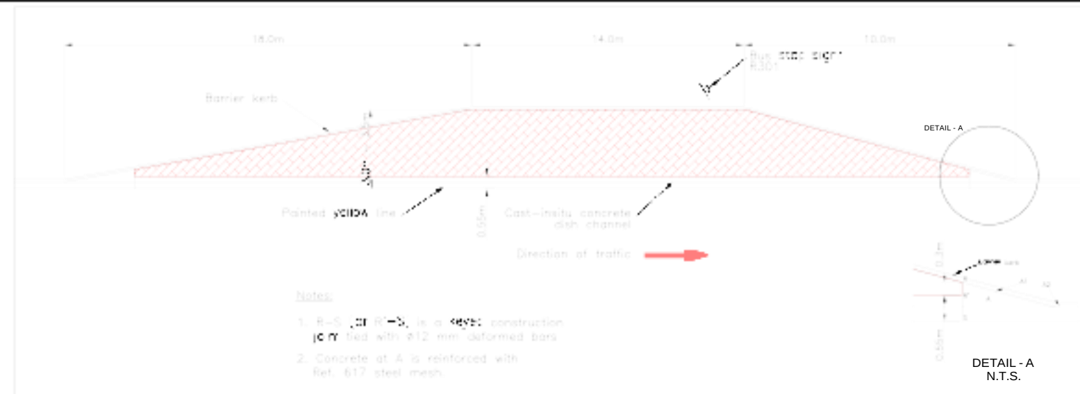
GEOMETRICAL LAYOUT OF BUS BAY FOR SINGLE BUS - USING CAST-IN SITU DISH CHANNEL SCALE - 1: 100
