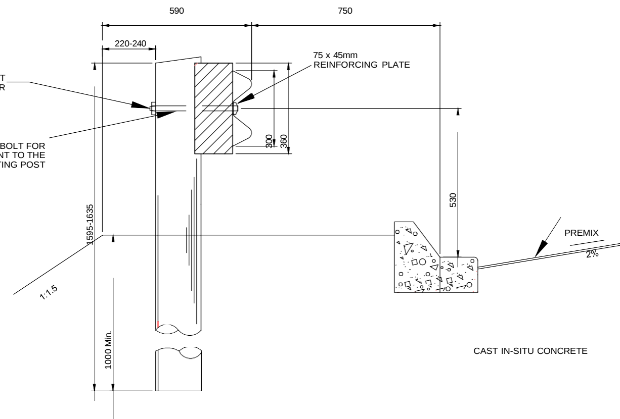
SIDE ELEVATION 1:10
