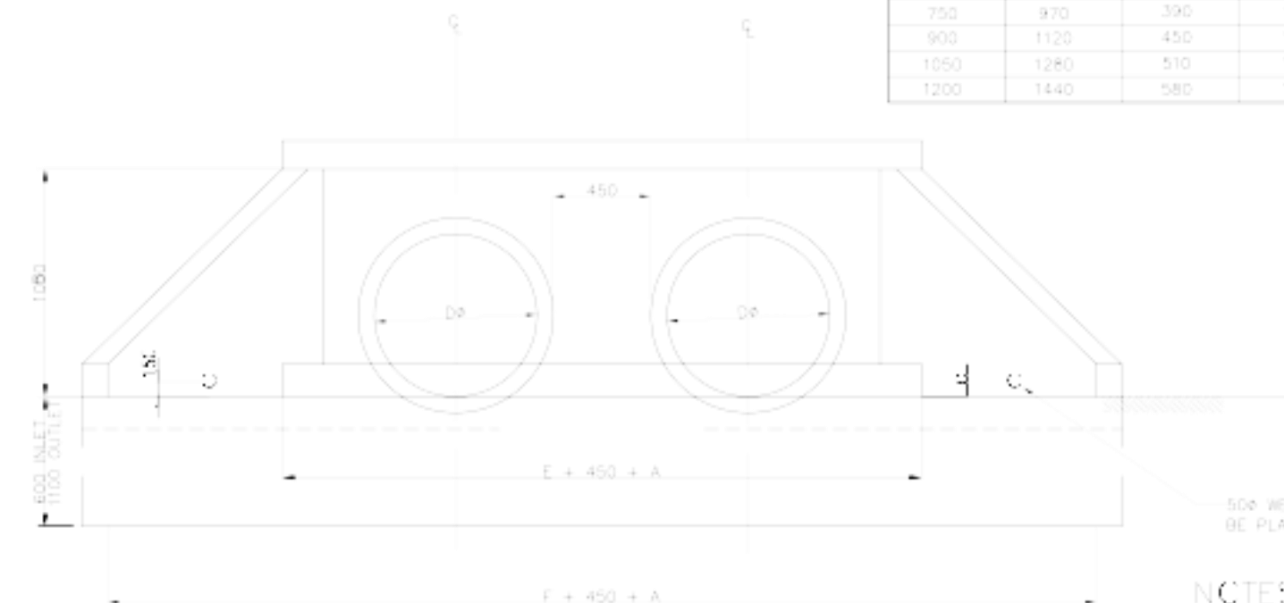
FRONT ELEVATION - MULTIPLE PIPES (FOR DIMENSIONS SEE TABLE 1) SCALE 1:20
