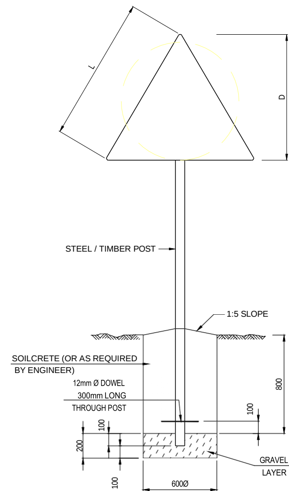
FOUNDATION DETAIL
