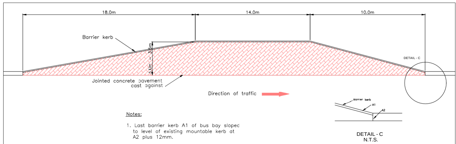
GEOMETRICAL LAYOUT OF BUS BAY FOR SINGLE BUS - USING JOINTED PAVEMENT SCALE - 1: 100
