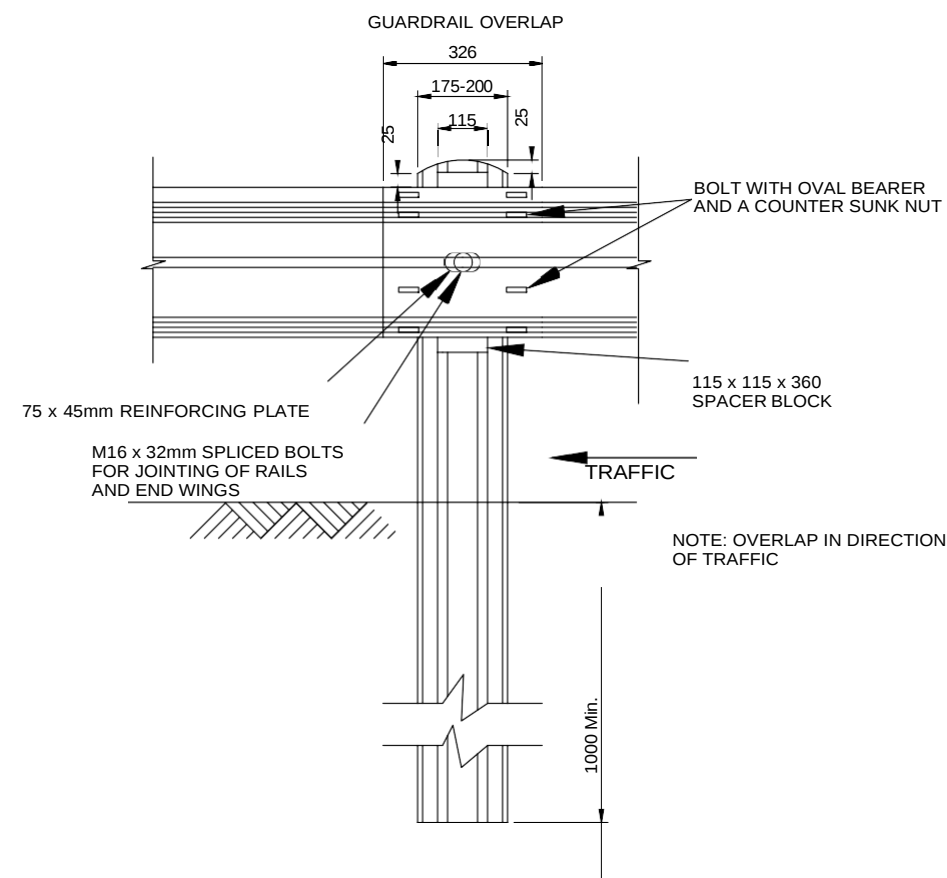
FRONT ELEVATION OF OVERLAP
