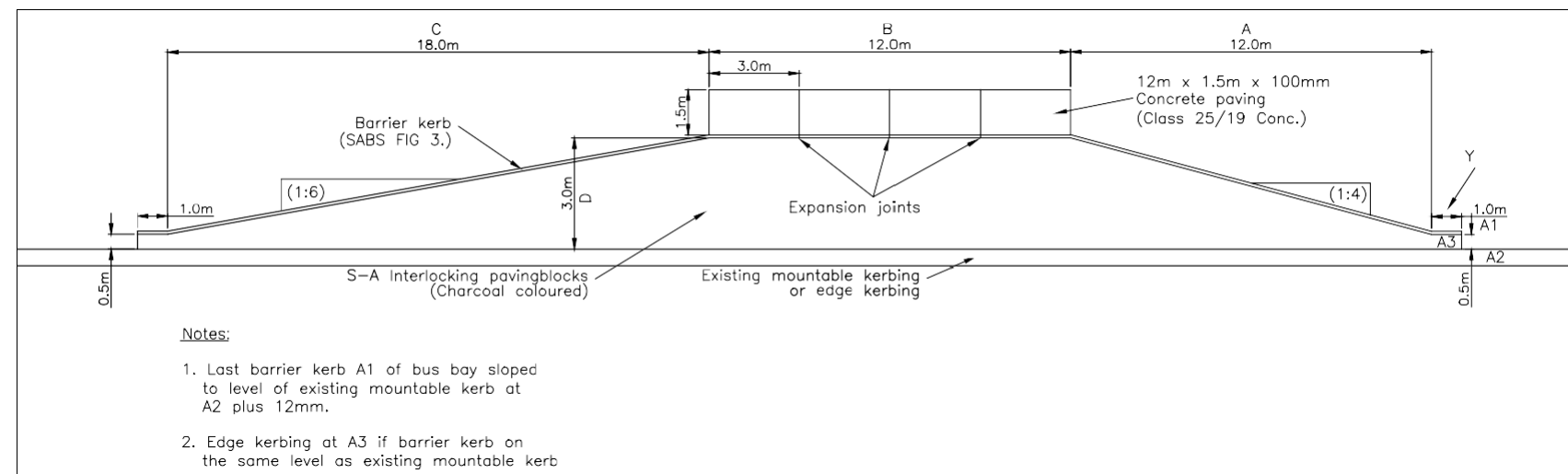
LAYOUT PLAN OF TYPICAL BUS BAY SCALE - 1: 150
