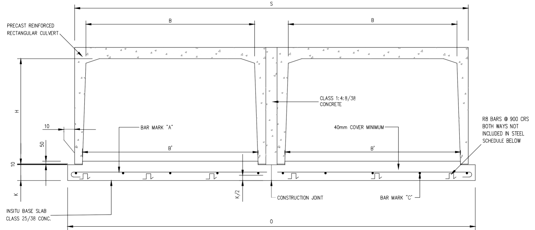
TYPICAL CROSS SECTION : MULTIPLE UNITS SCALE 1:20
