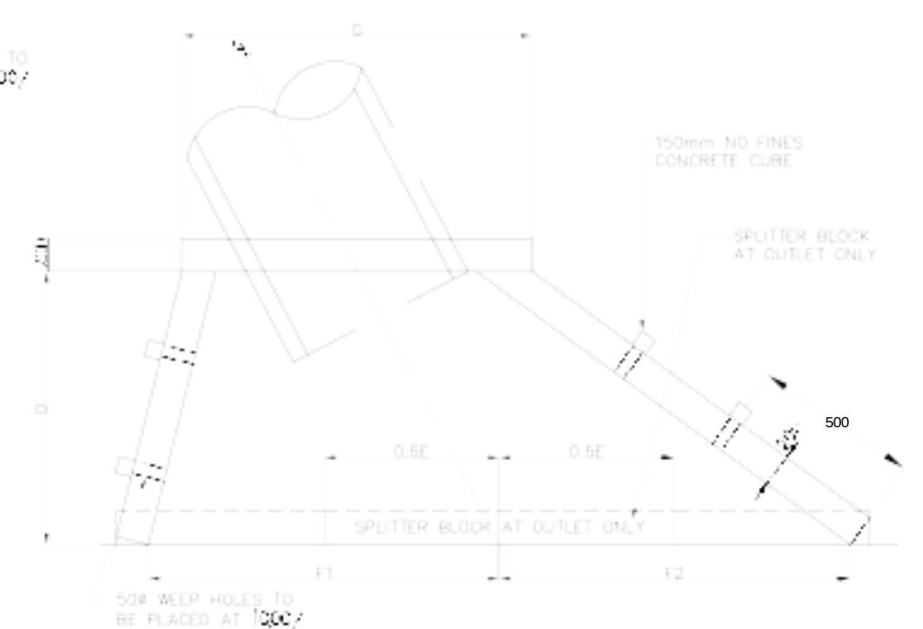
SKEW PIPE CULVERT (FOR DIMENSIONS SEE TABLE 3) SCALE 1:20
