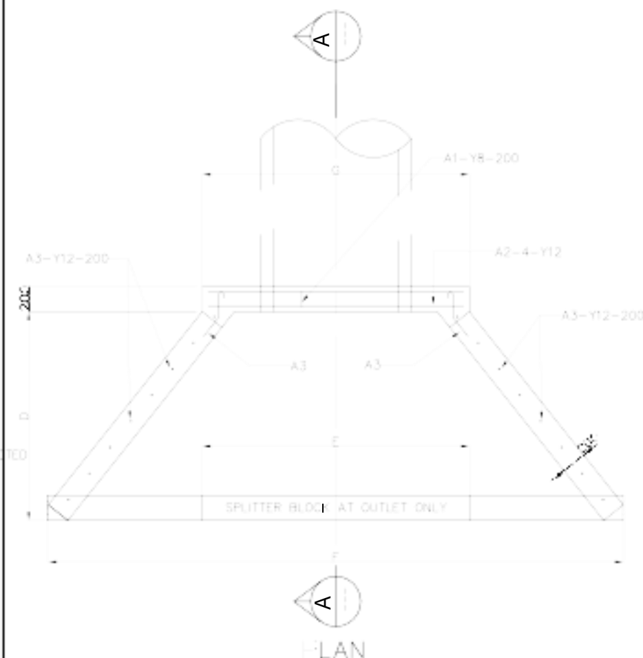
(FOR DIMENSIONS SEE TABLE 1) (FOR REINFORCEMENT SEE TABLE 2) SCALE 1:20
