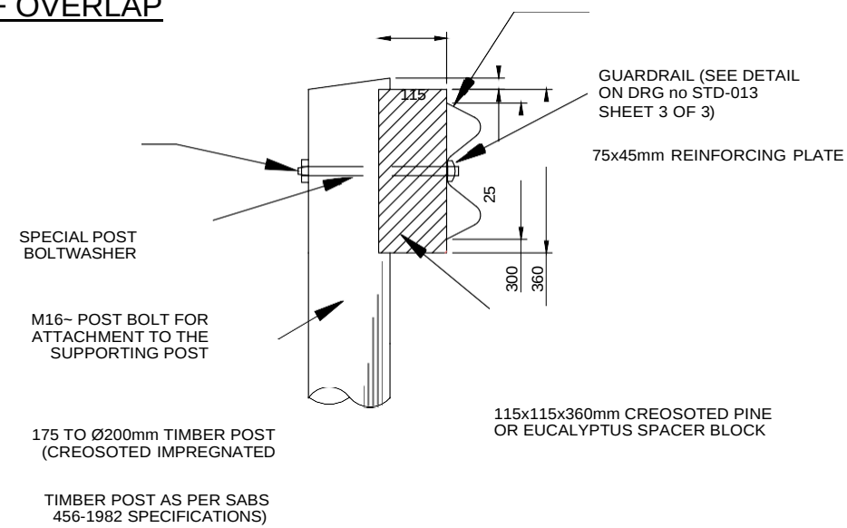
DETAIL OF FIXING SCALE 1:10
