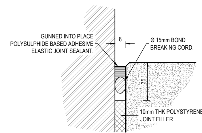
ISOLATION JOINT DETAIL (I.J.) SCALE 1:2
