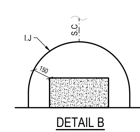
DETAIL B SCALE 1:20
