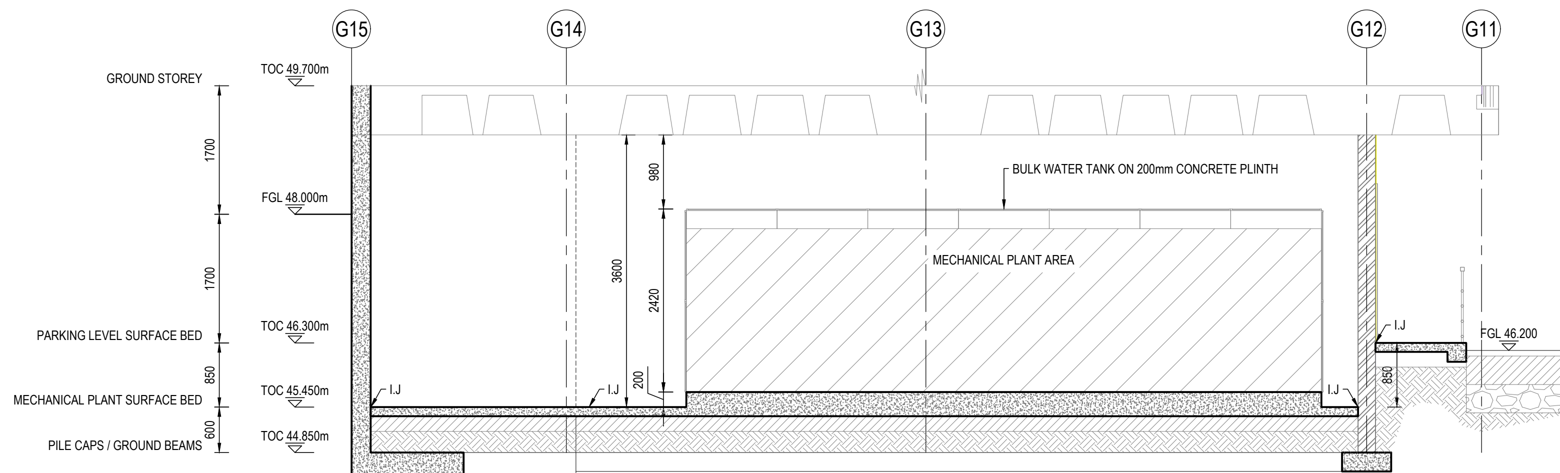
SECTION X SCALE 1:50
