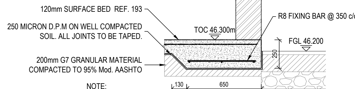
SLAB EDGE THICKENING: SCALE 1:20
