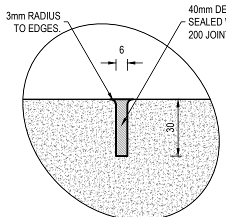
SAW CUT JOINT DETAIL (S.C.) SCALE 1:2
