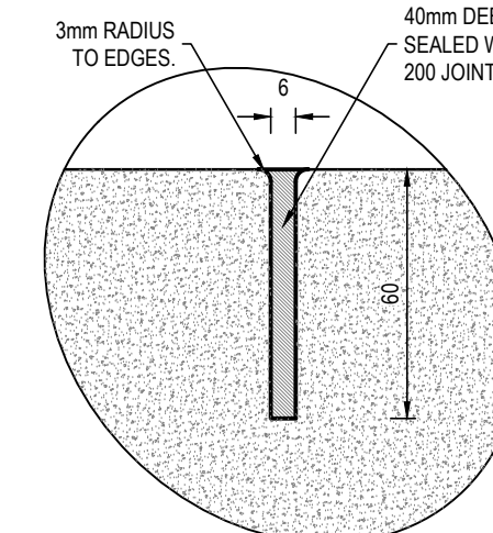
LONGITUDINAL SAW CUT JOINT DETAIL (L.S.C.) SCALE 1:2
