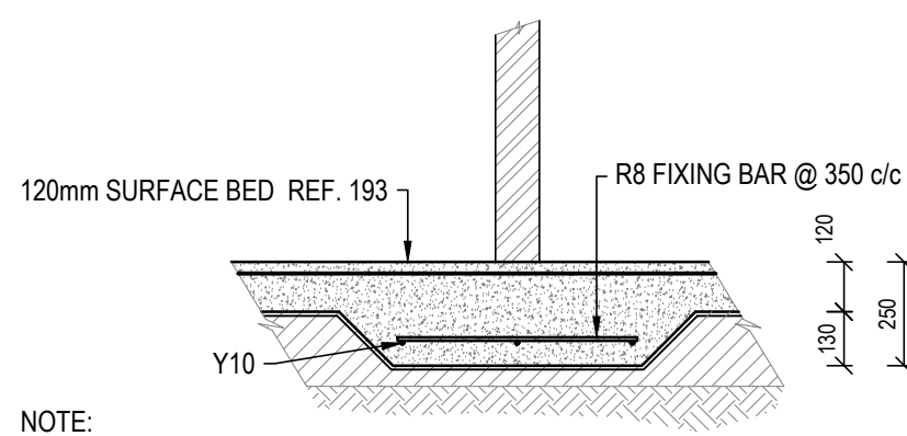
SLAB THICKENING: SCALE 1:20
